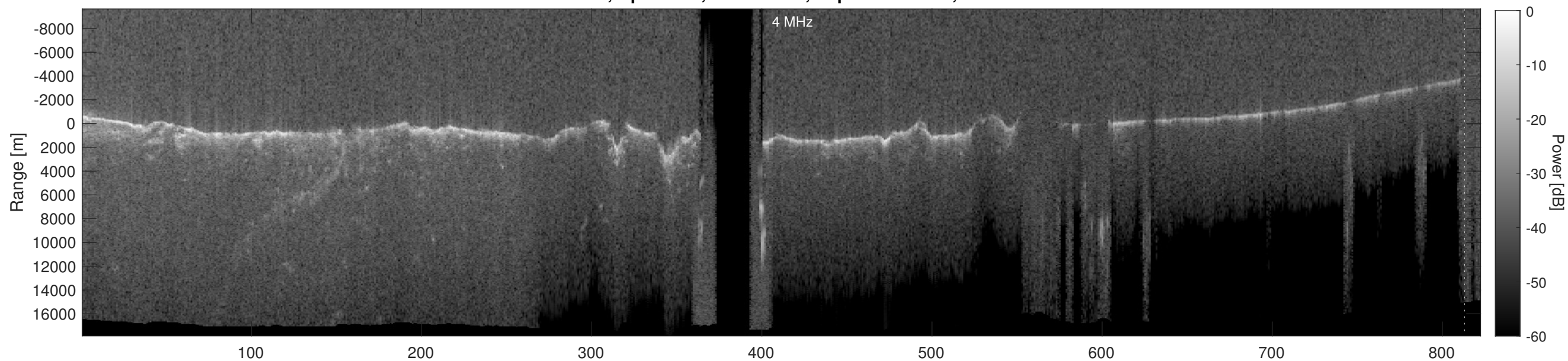
Orbit 14678, Depth-Corrected Cluttergram
