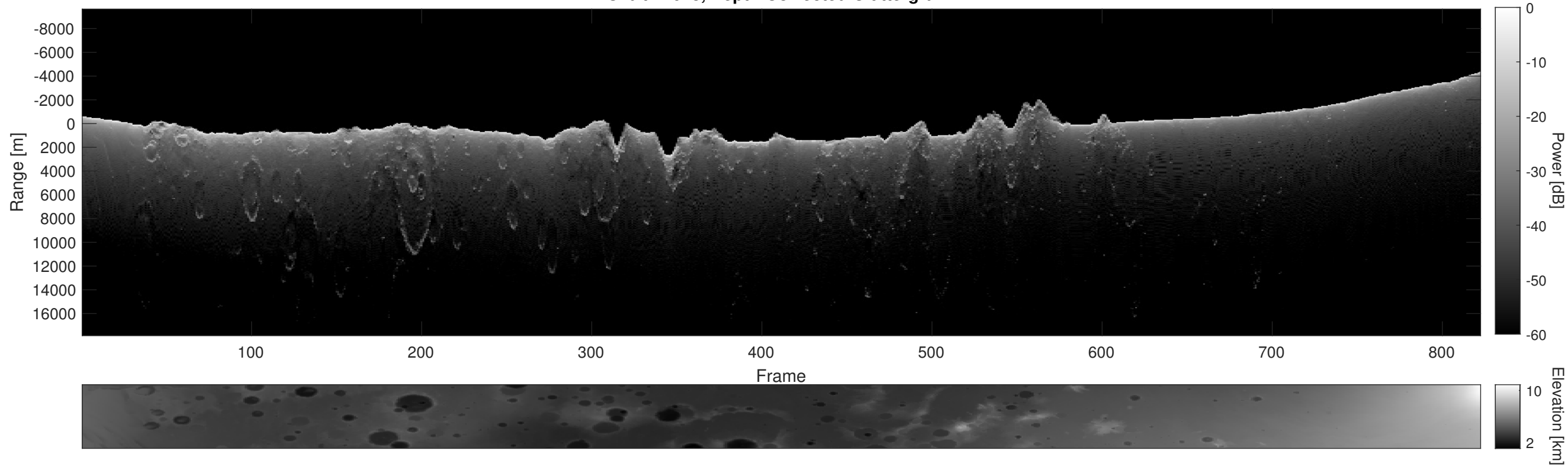
Orbit 14678, Depth-Corrected Cluttergram
