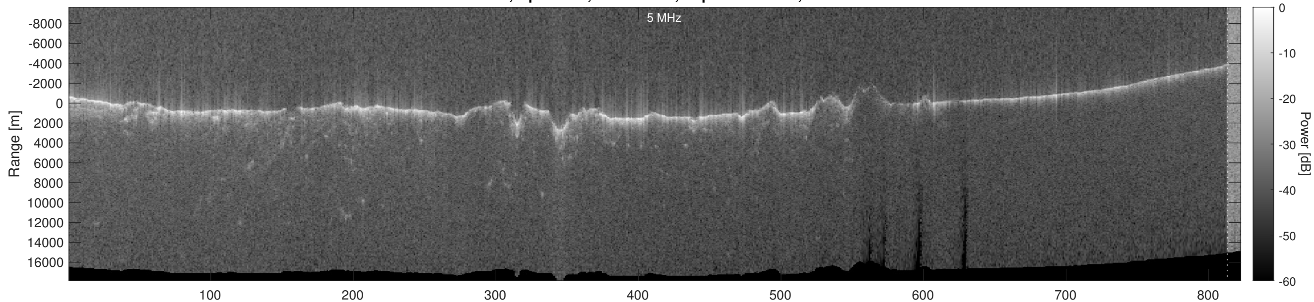
Orbit 14678, Optimized, No Window, Depth-Corrected, Channel 2
