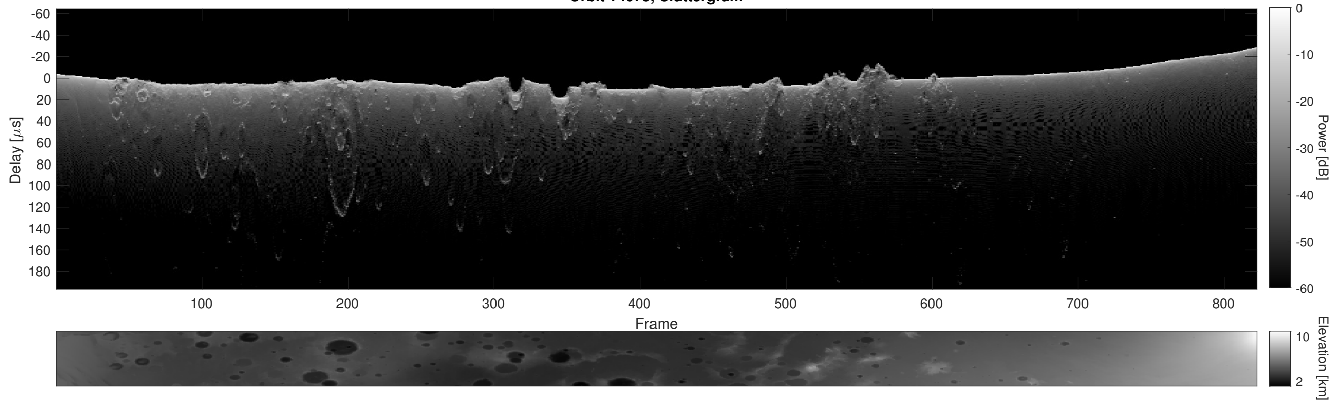
Orbit 14678, Cluttergram
