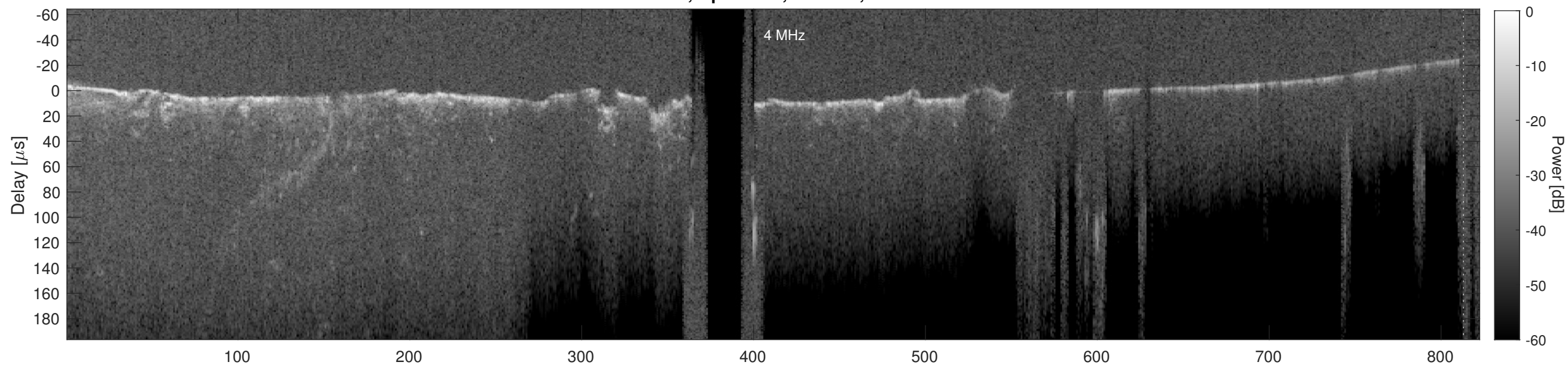
Orbit 14678, Cluttergram
