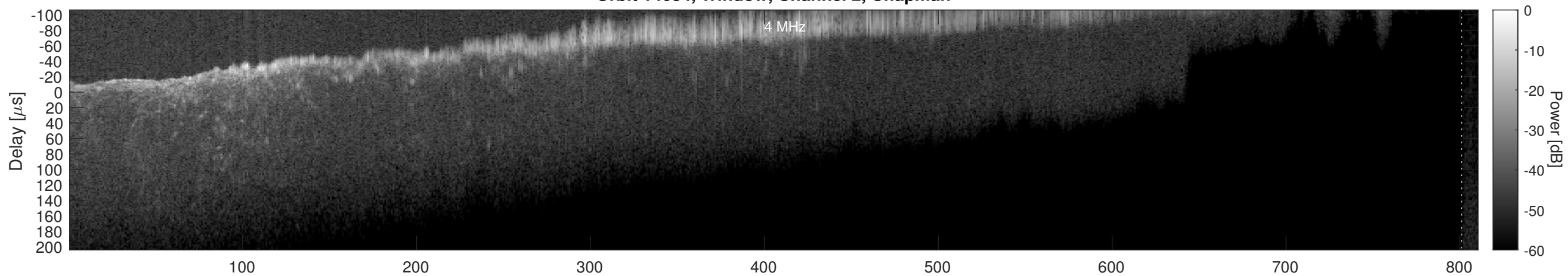
Orbit 14684, Window, Channel 2, Optimized
