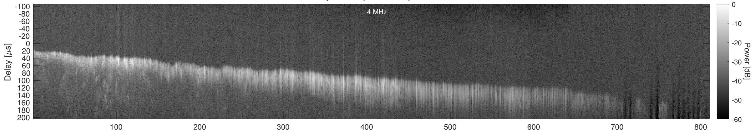
Orbit 14684, Window, Channel 2, Chapman
