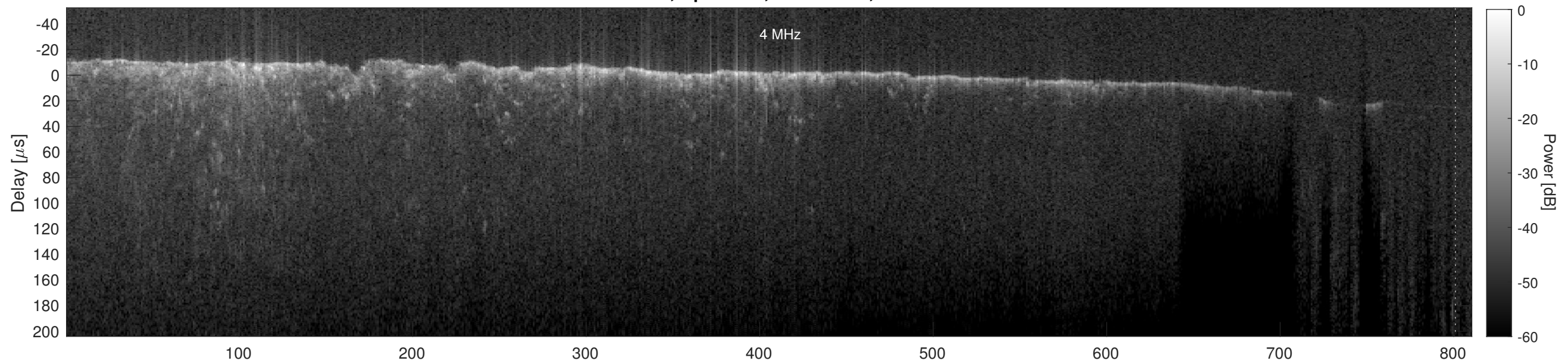
Orbit 14684, Cluttergram
