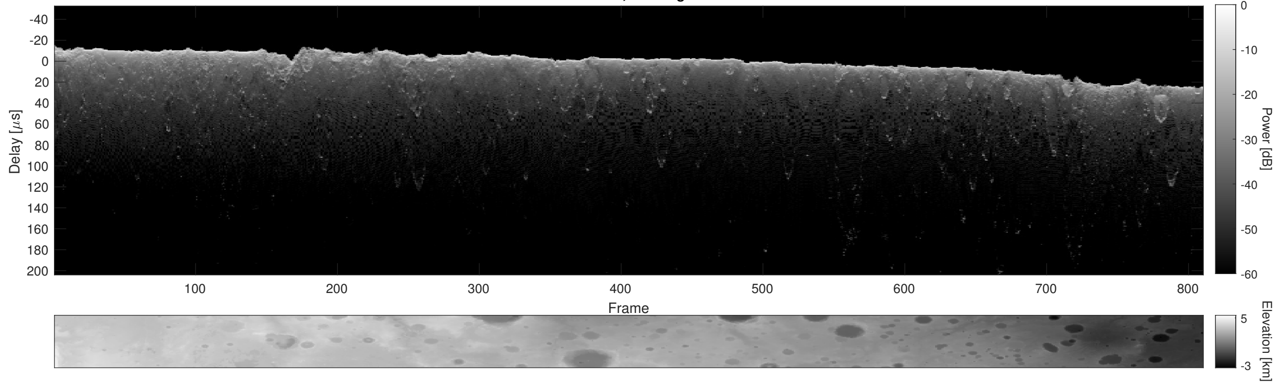
Orbit 14684, Cluttergram
