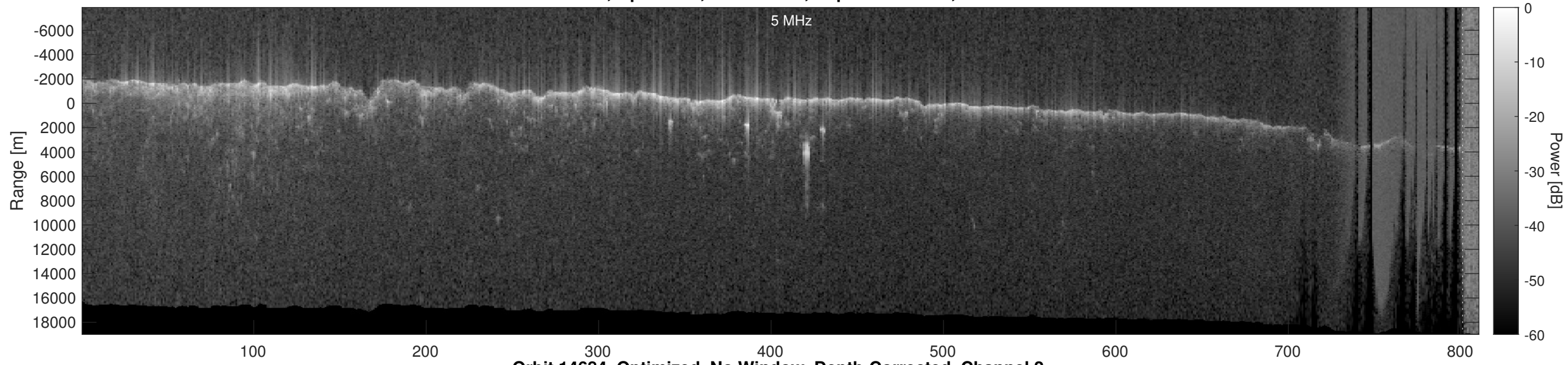
Orbit 14684, Optimized, No Window, Depth-Corrected, Channel 2
