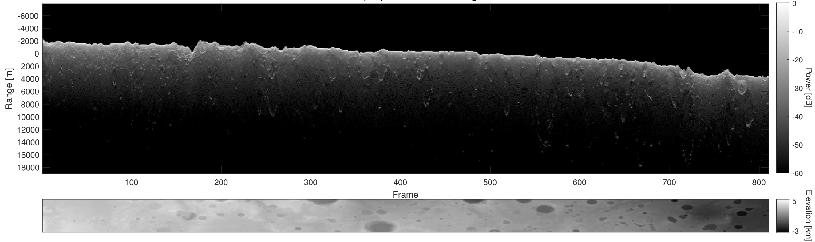
Orbit 14684, Depth-Corrected Cluttergram
