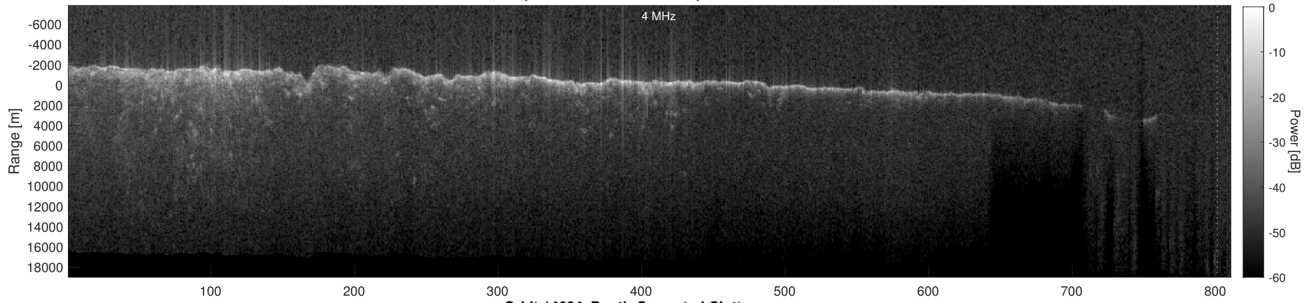
Orbit 14684, Depth-Corrected Cluttergram
