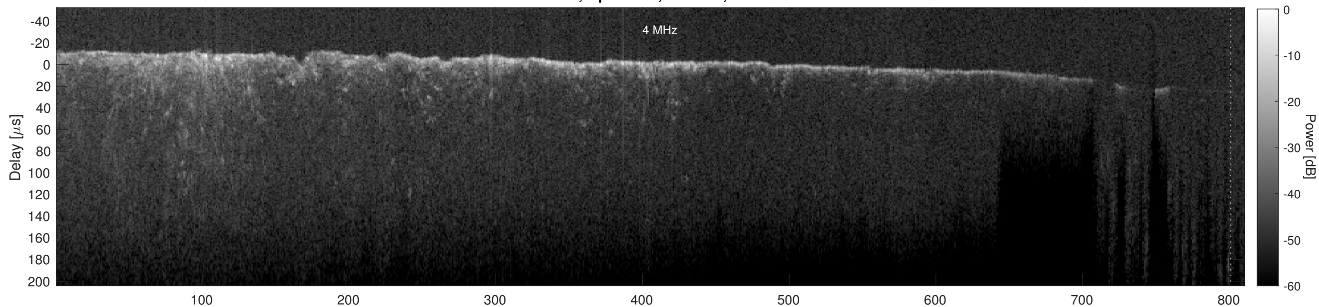
Orbit 14684, Cluttergram
