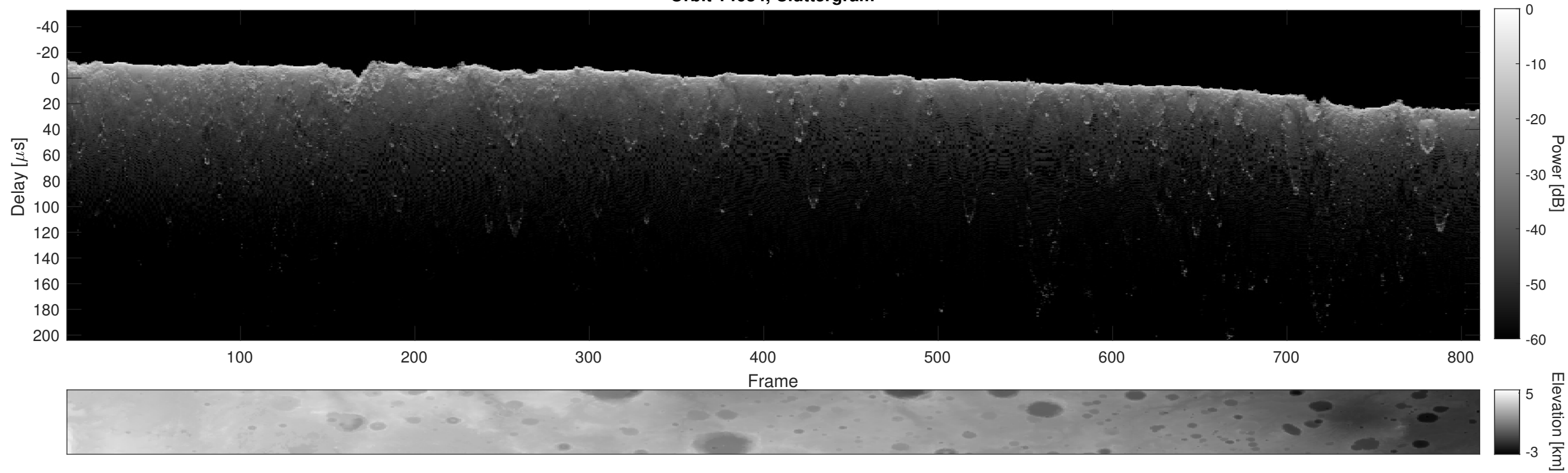
Orbit 14684, Cluttergram
