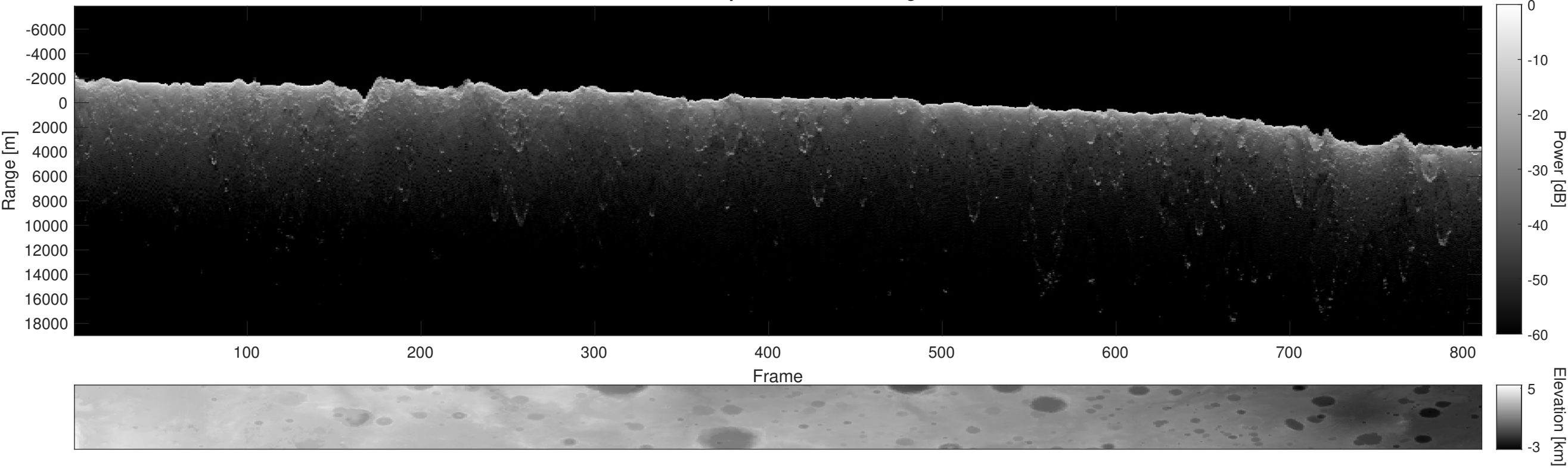
Orbit 14684, Depth-Corrected Cluttergram
