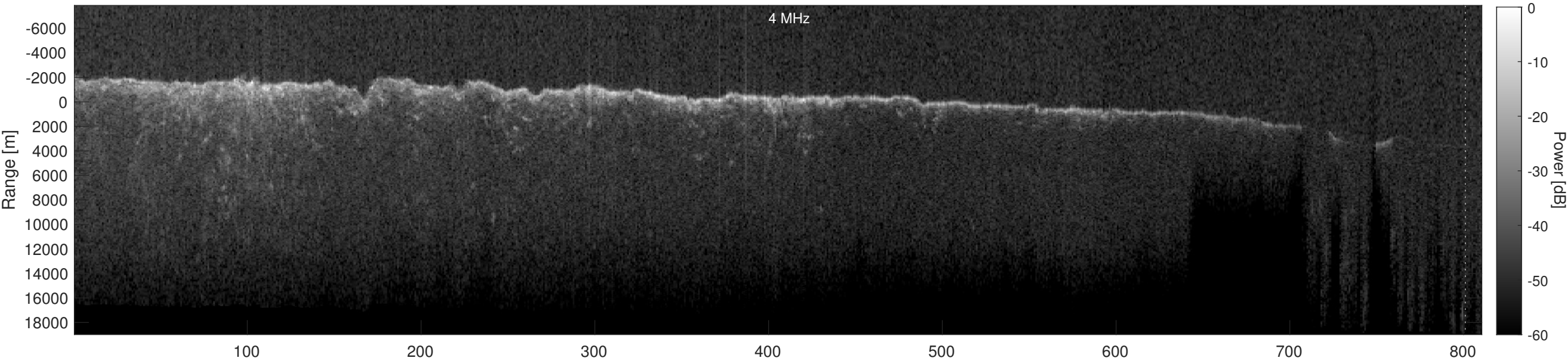
Orbit 14684, Depth-Corrected Cluttergram
