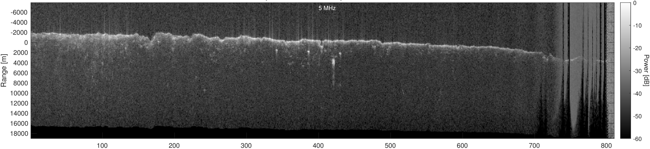
Orbit 14684, Optimized, Window, Depth-Corrected, Channel 2
