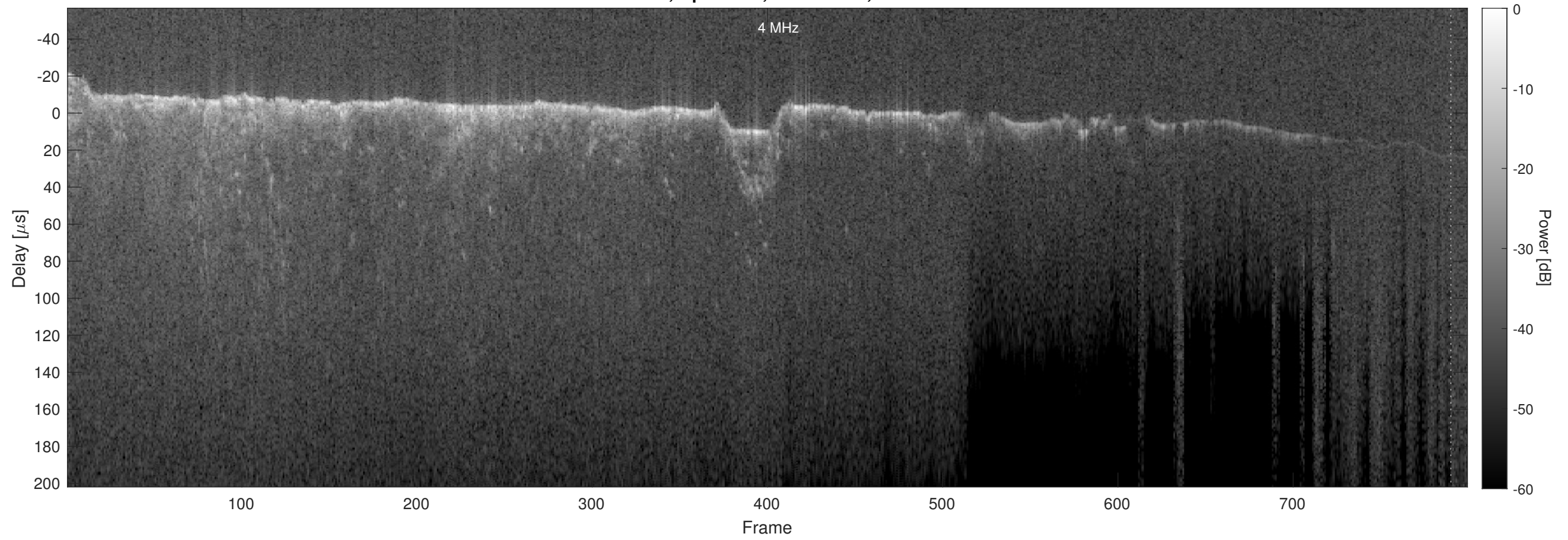
Orbit 14691, Optimized, No Window, Channel 2
