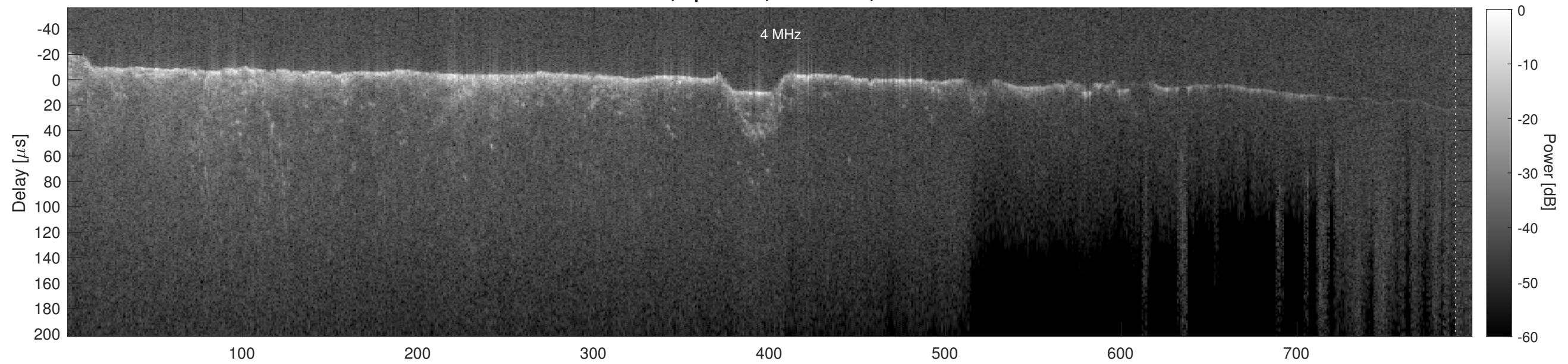
Orbit 14691, Cluttergram
