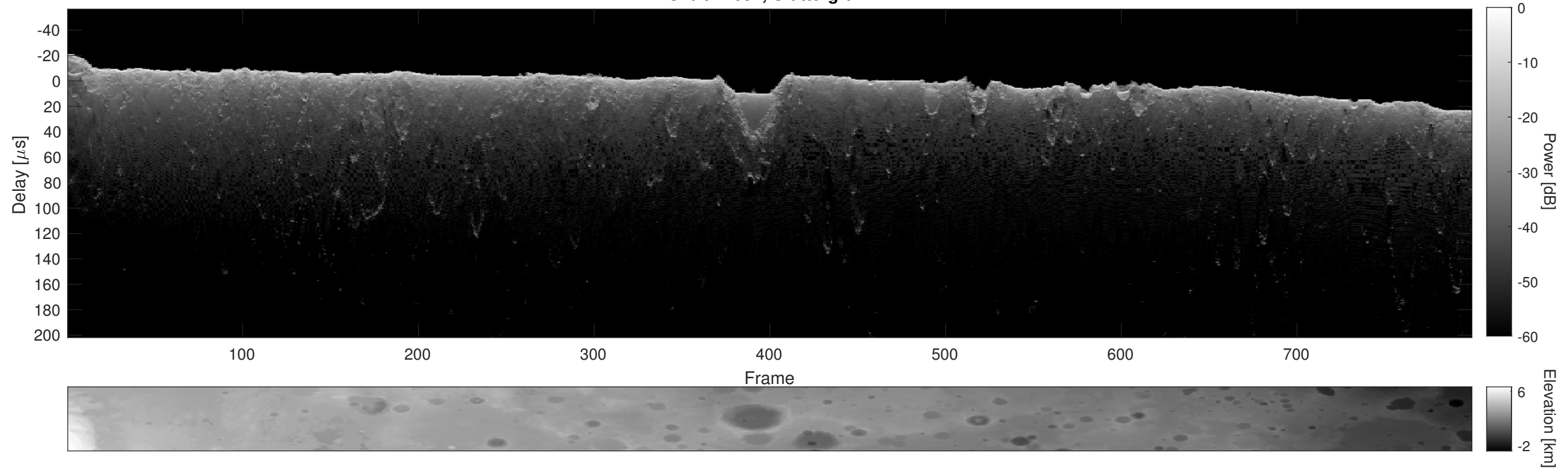
Orbit 14691, Cluttergram
