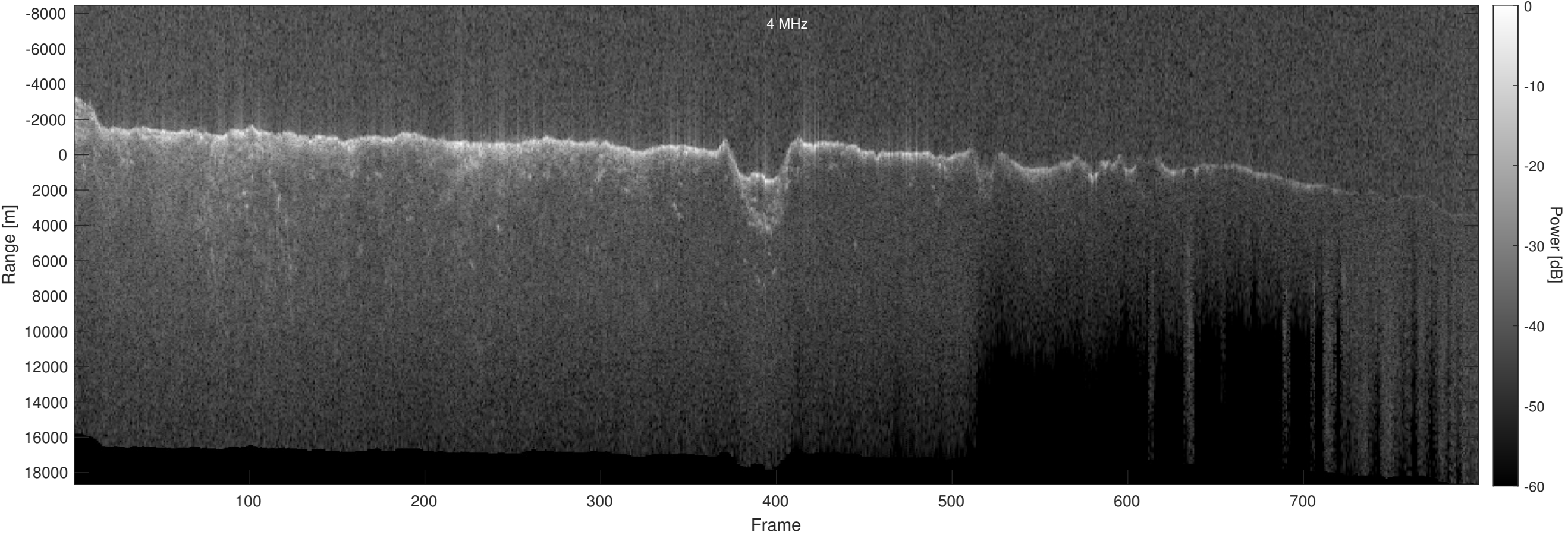
Orbit 14691, Optimized, No Window, Depth-Corrected, Channel 2
