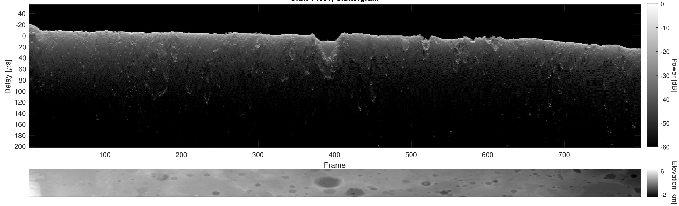
Orbit 14691, Cluttergram
