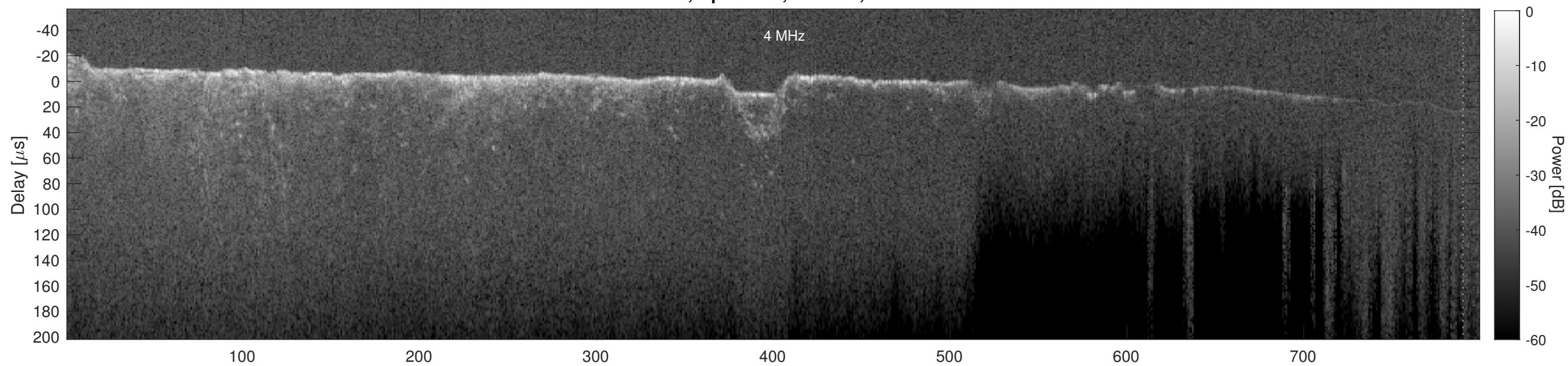
Orbit 14691, Cluttergram
