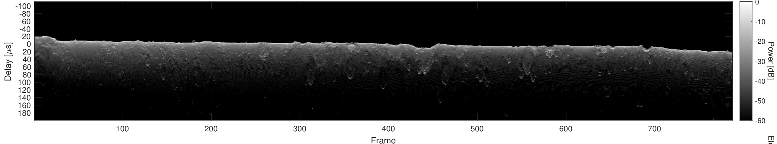
Orbit 14698, Cluttergram
