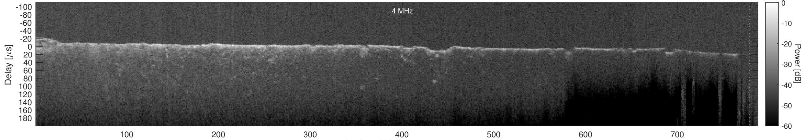
Orbit 14698, Cluttergram
