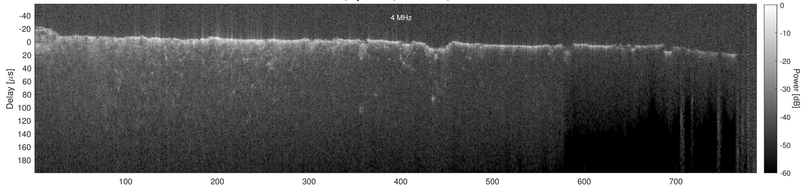
Orbit 14698, Cluttergram
