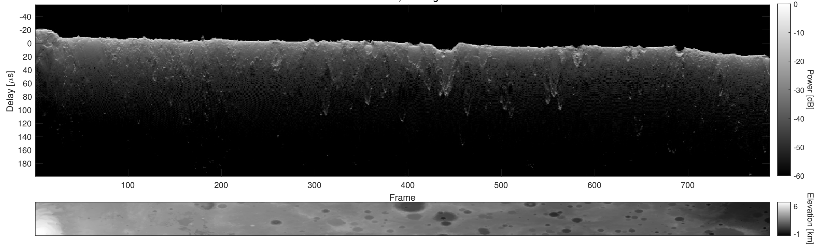
Orbit 14698, Cluttergram
