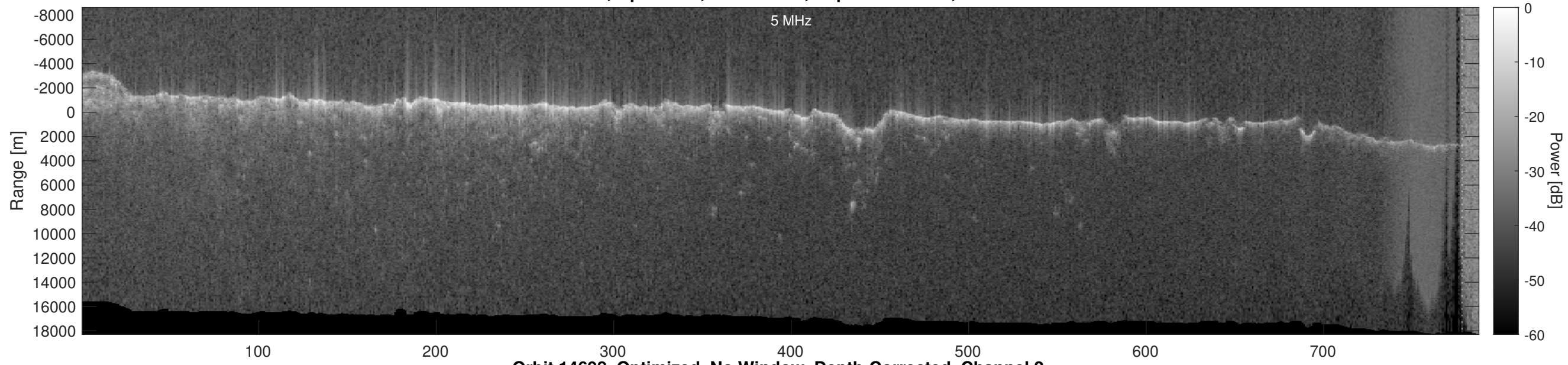
Orbit 14698, Optimized, No Window, Depth-Corrected, Channel 2
