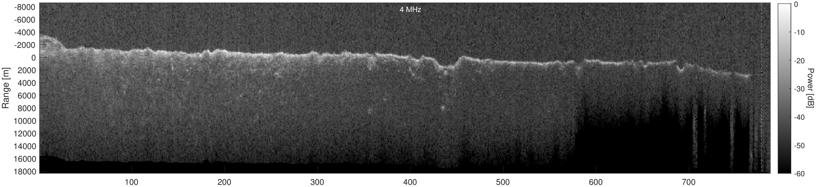
Orbit 14698, Depth-Corrected Cluttergram
