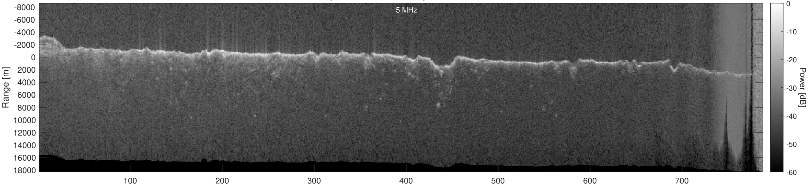
Orbit 14698, Optimized, Window, Depth-Corrected, Channel 2
