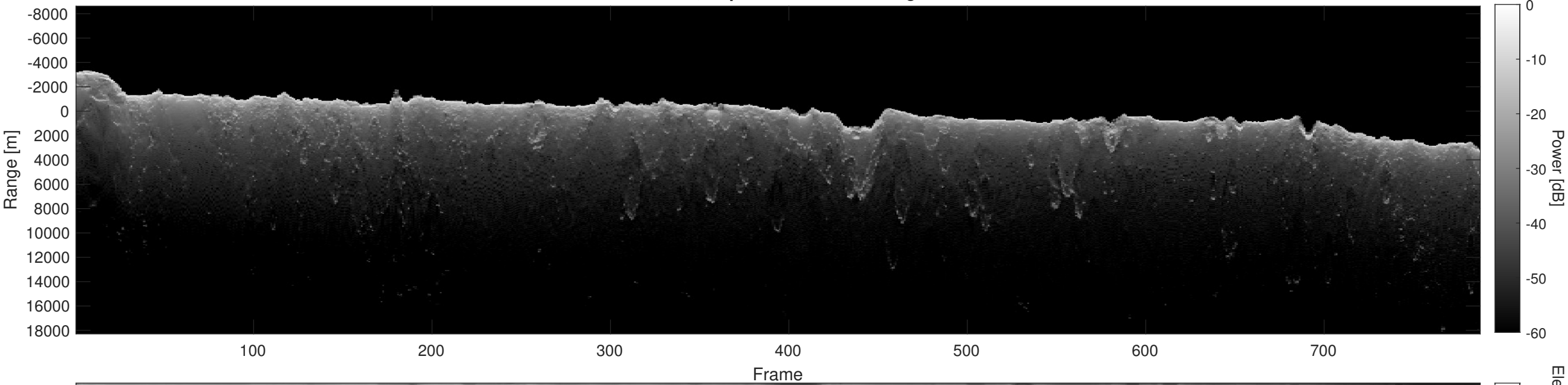
Orbit 14698, Depth-Corrected Cluttergram
