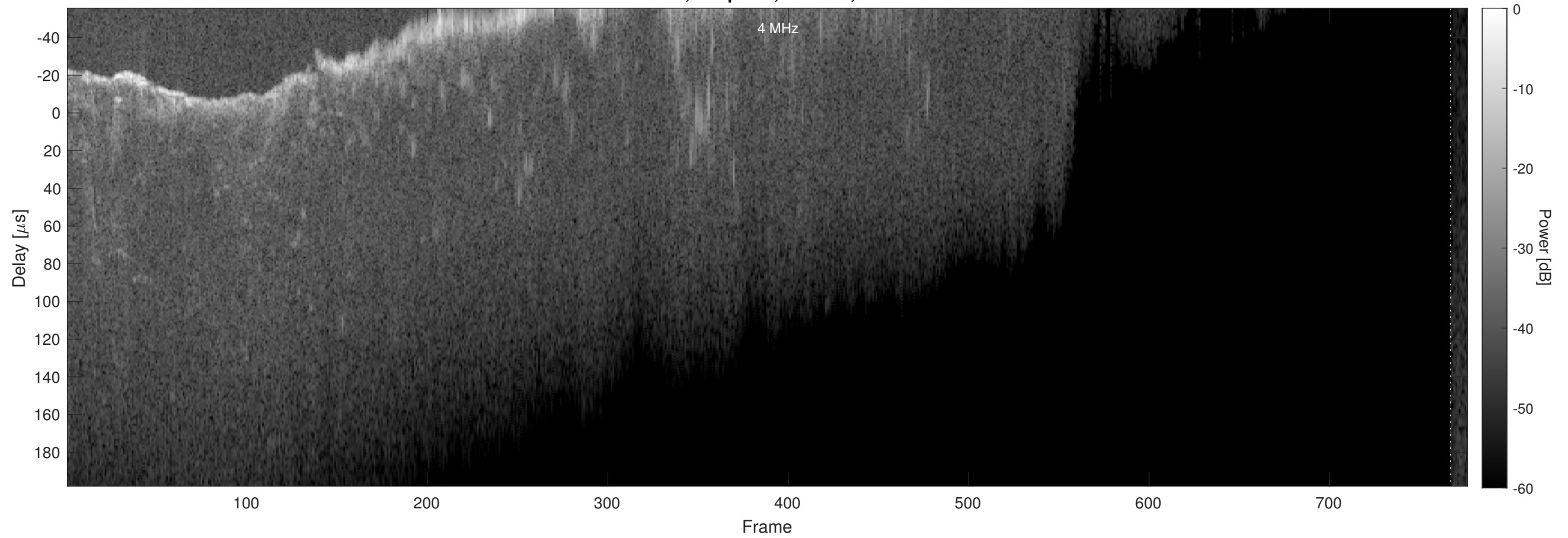
Orbit 14704, Chapman, Window, Channel 2
