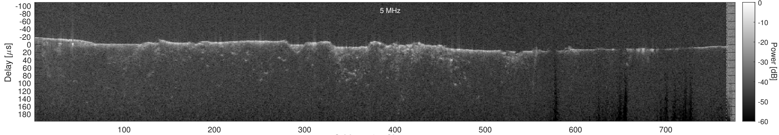
Orbit 14704, Cluttergram
