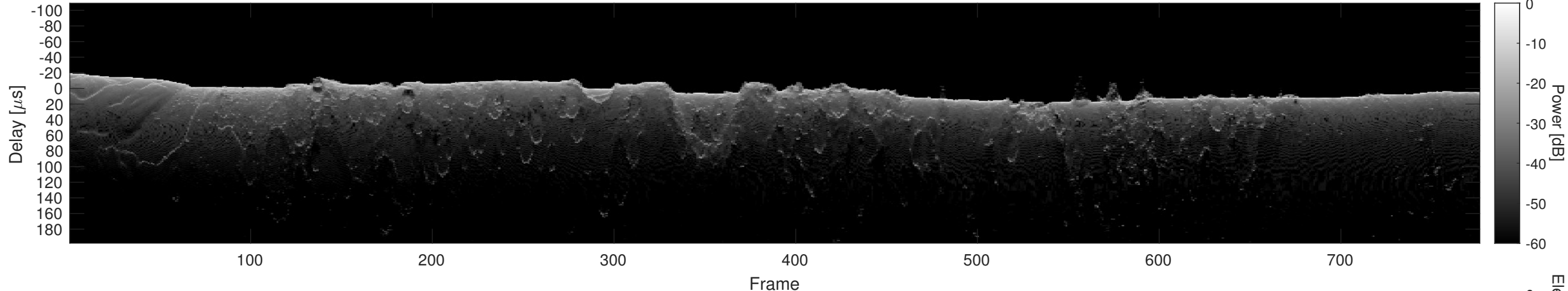
Orbit 14704, Cluttergram
