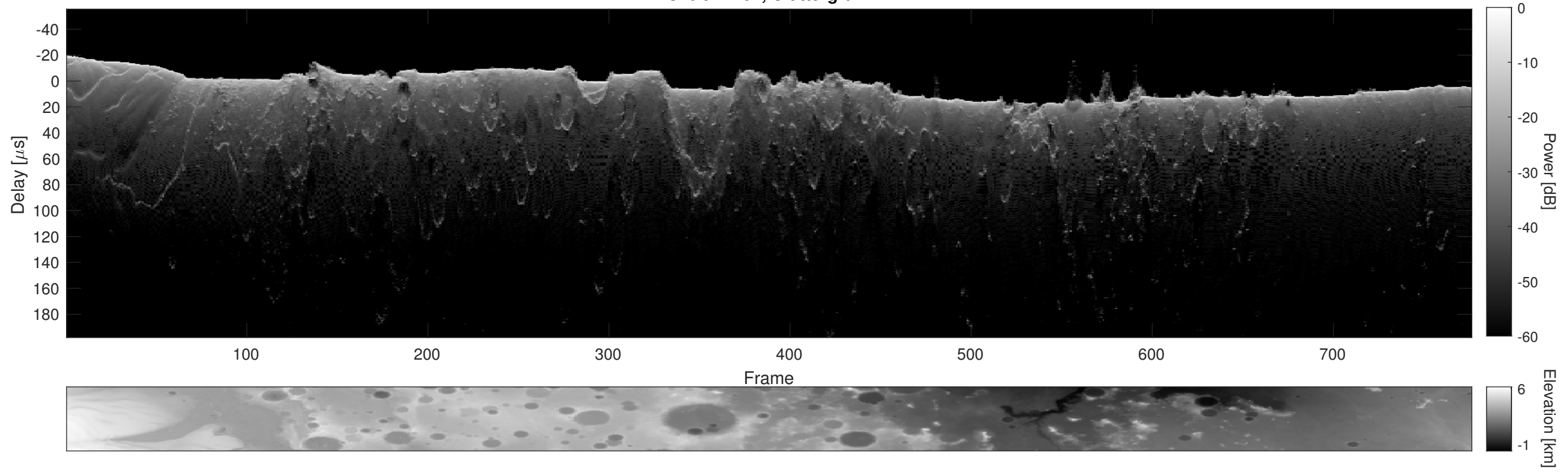
Orbit 14704, Cluttergram
