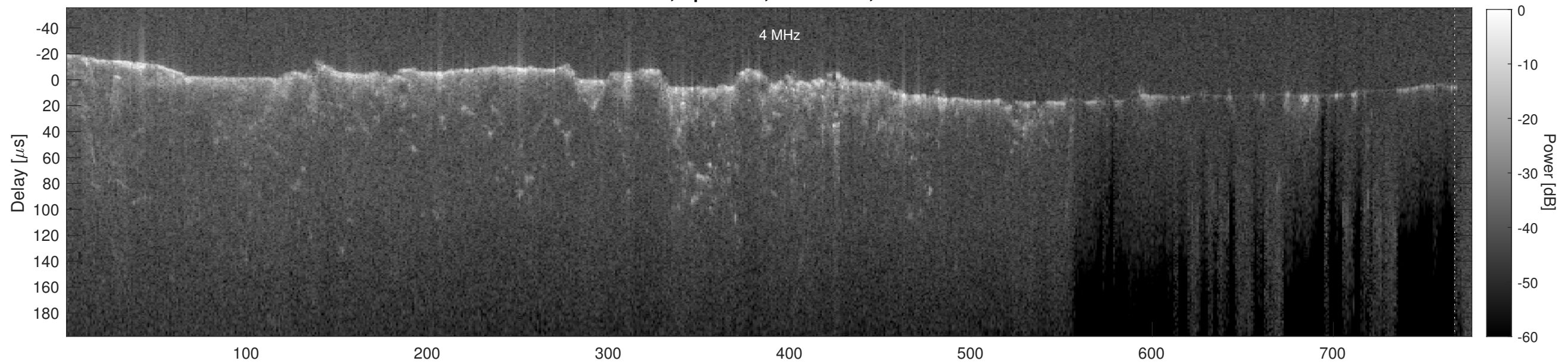
Orbit 14704, Cluttergram
