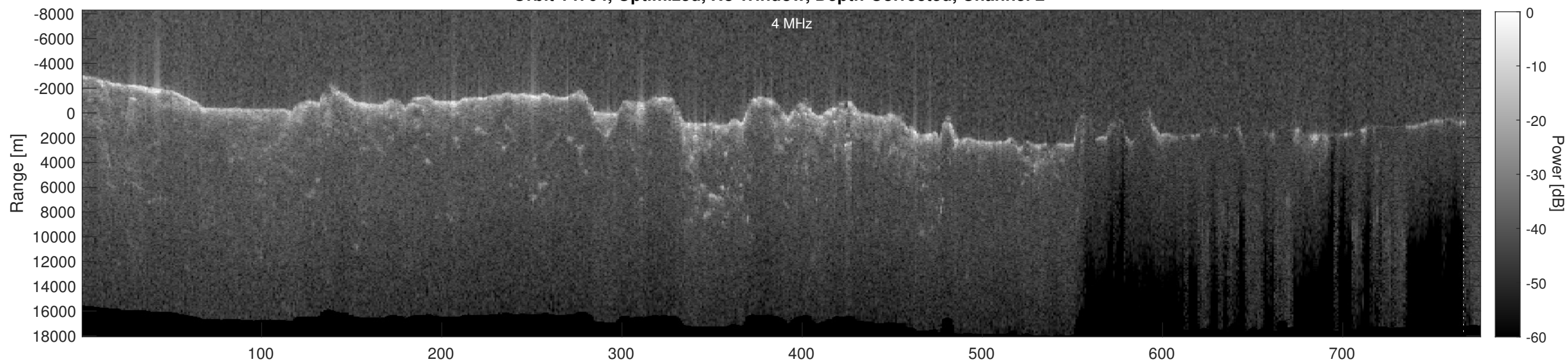
Orbit 14704, Depth-Corrected Cluttergram
