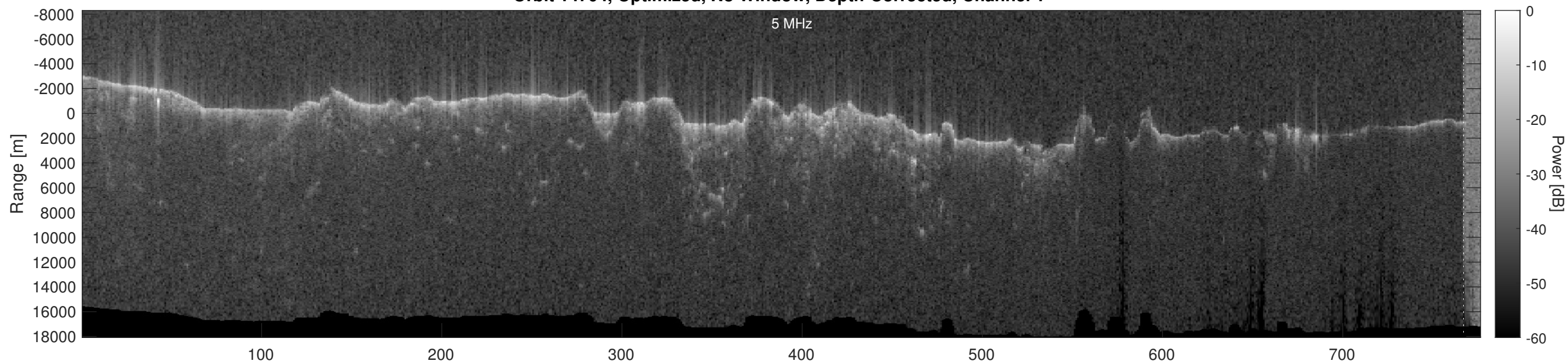
Orbit 14704, Optimized, No Window, Depth-Corrected, Channel 2
