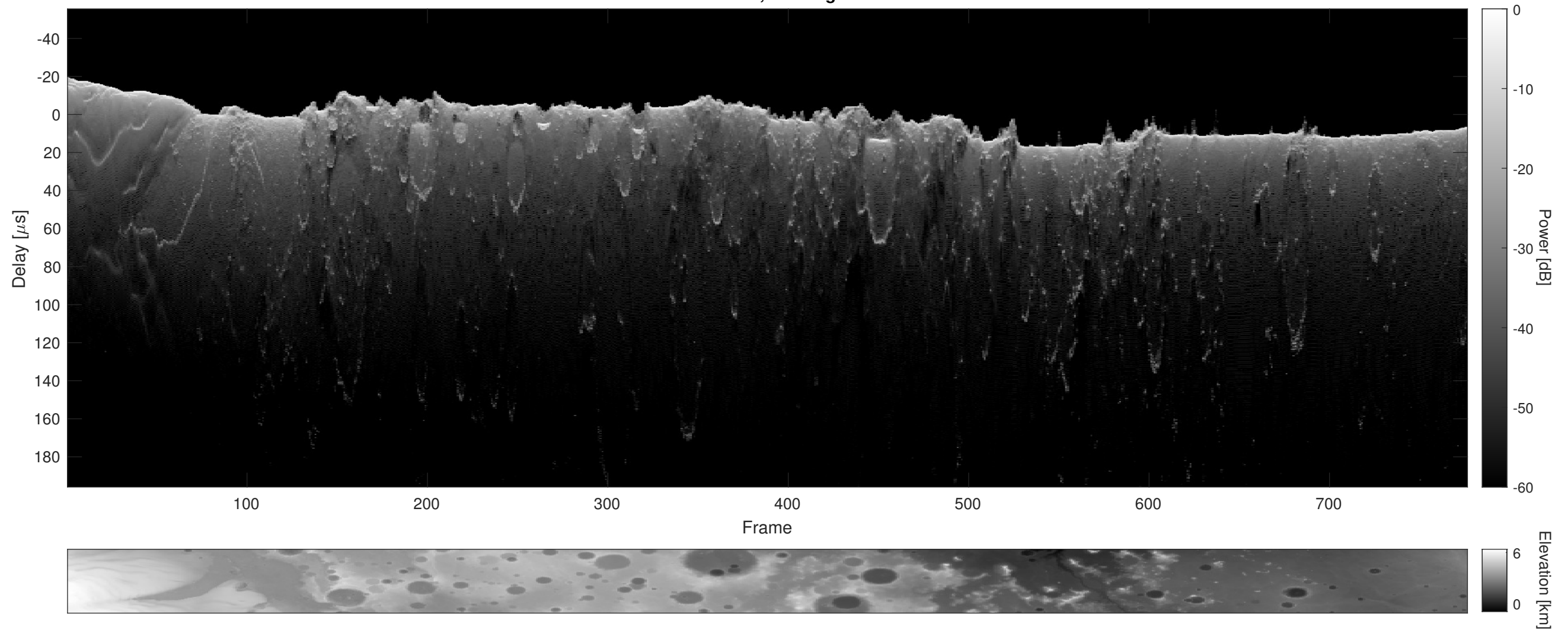
Orbit 14711, Cluttergram
