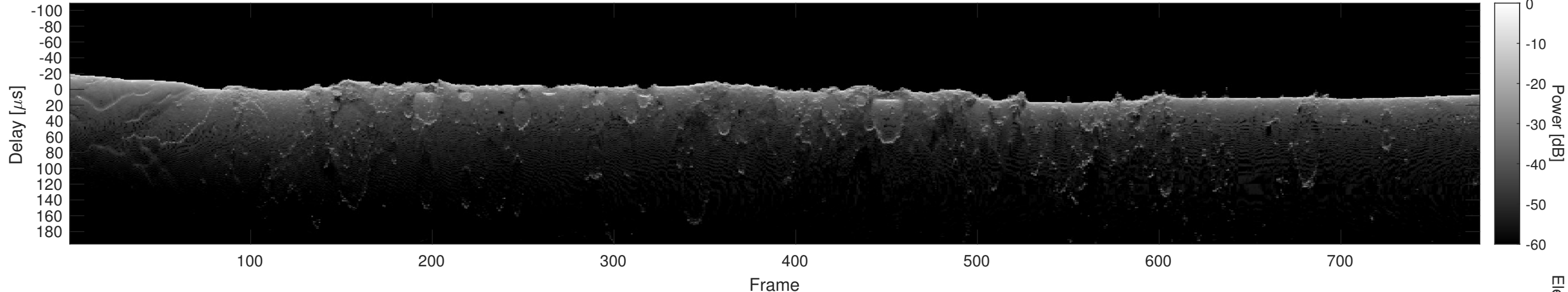
Orbit 14711, Cluttergram
