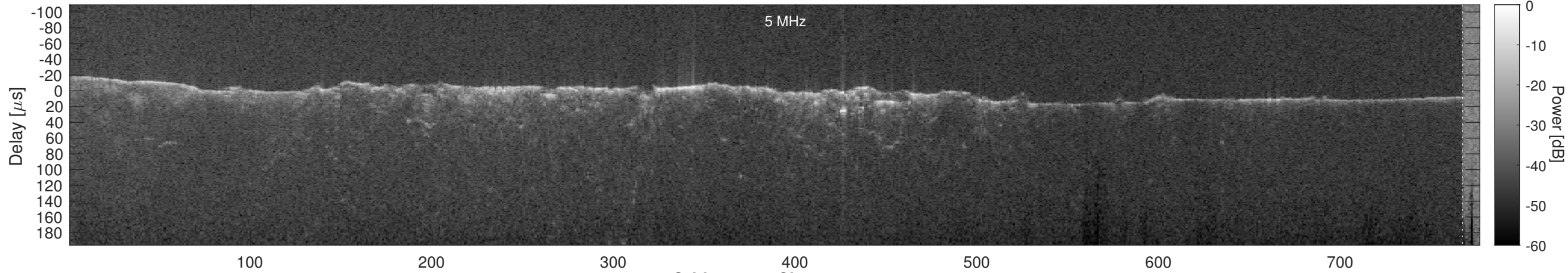
Orbit 14711, Cluttergram
