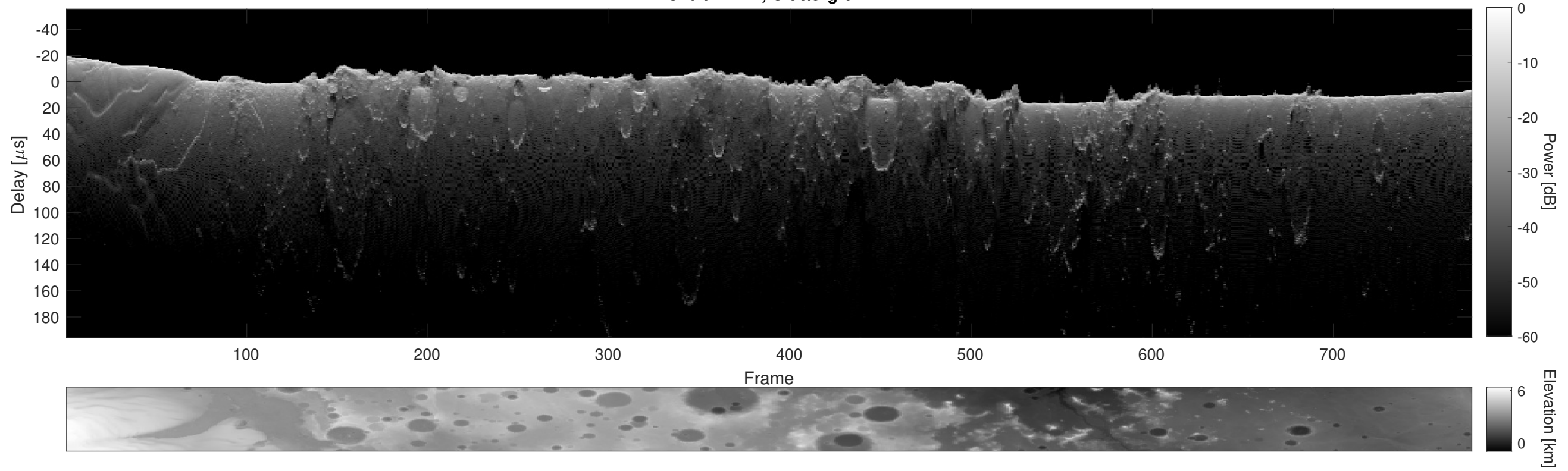
Orbit 14711, Cluttergram
