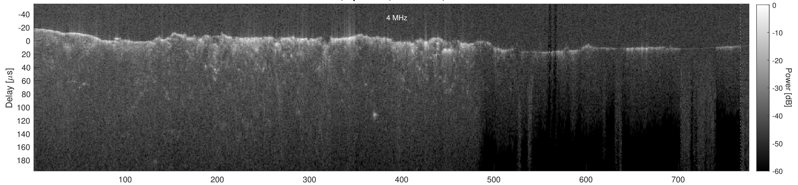
Orbit 14711, Cluttergram
