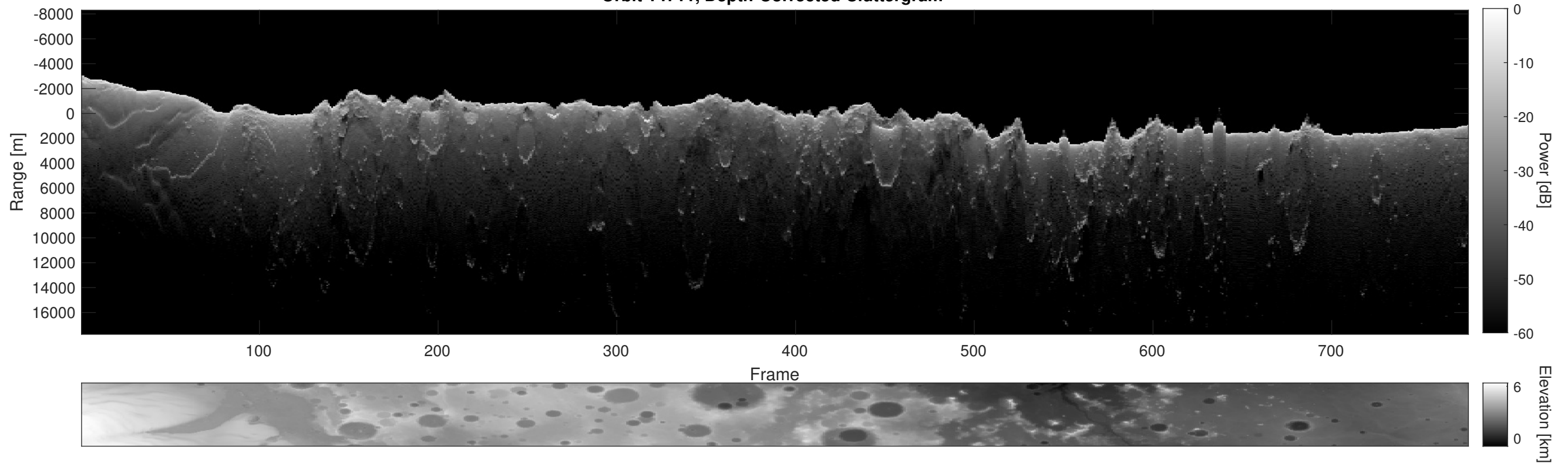
Orbit 14711, Depth-Corrected Cluttergram
