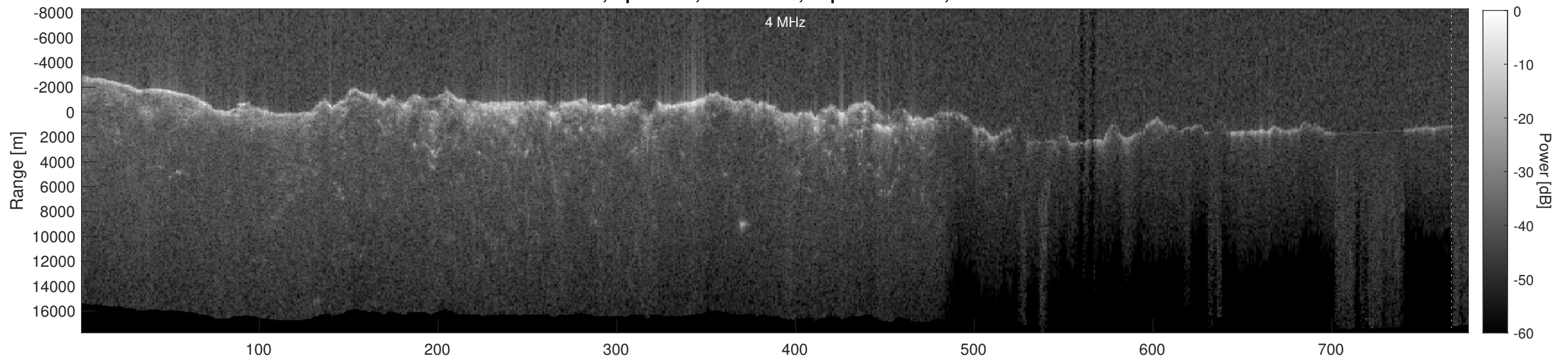
Orbit 14711, Depth-Corrected Cluttergram
