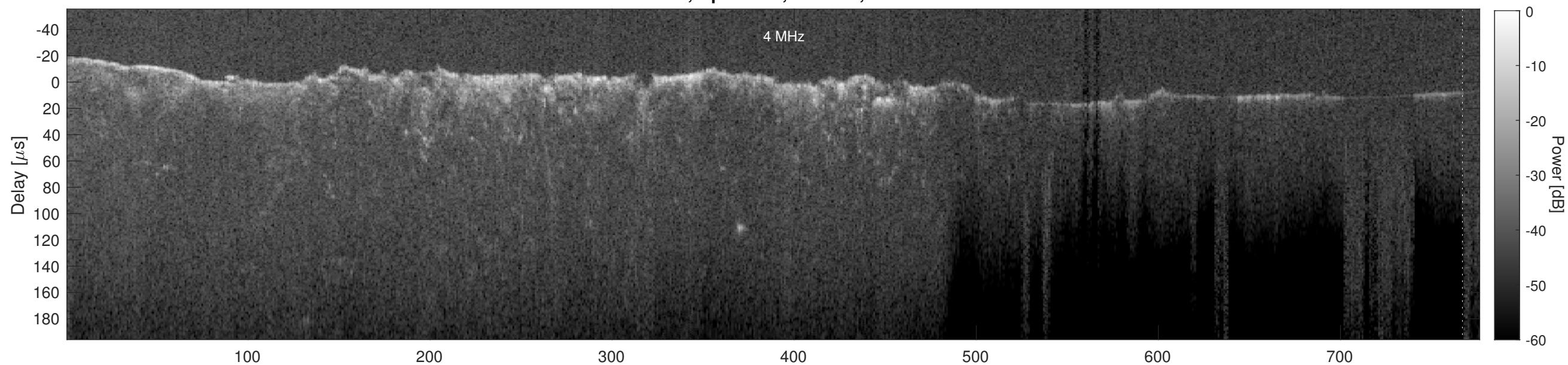
Orbit 14711, Cluttergram
