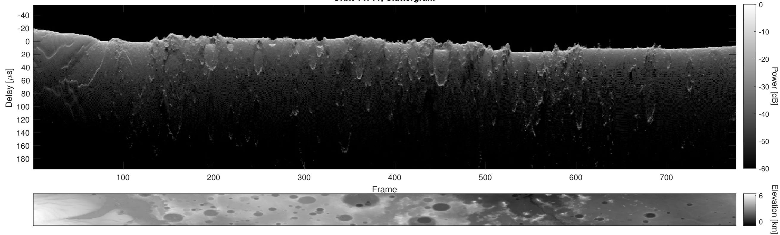
Orbit 14711, Cluttergram
