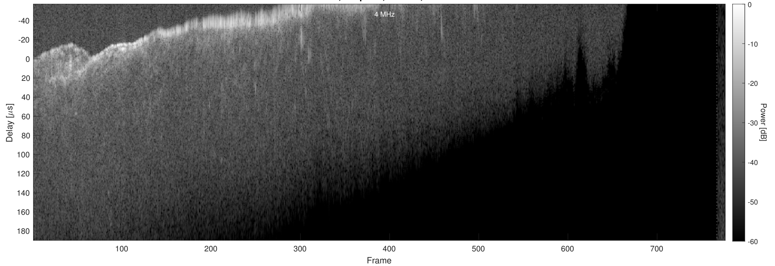
Orbit 14719, Chapman, Window, Channel 2
