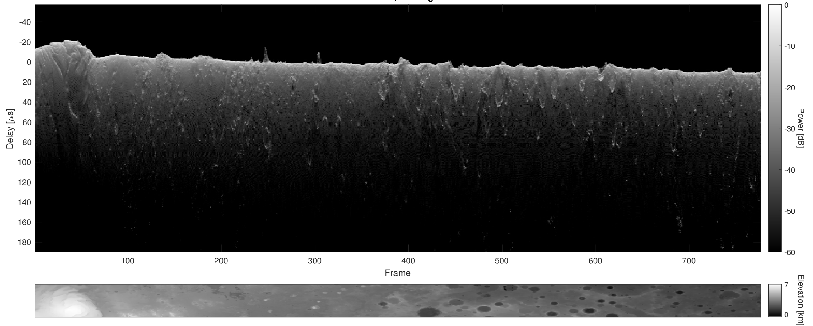
Orbit 14719, Cluttergram
