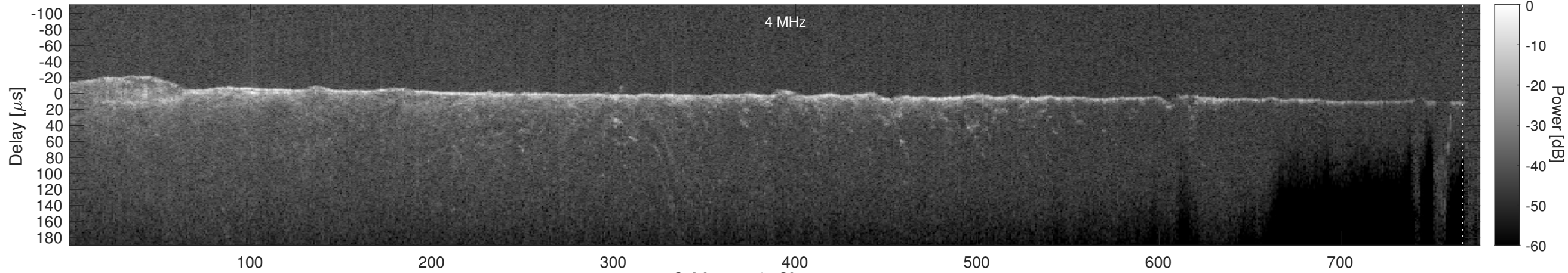
Orbit 14719, Cluttergram
