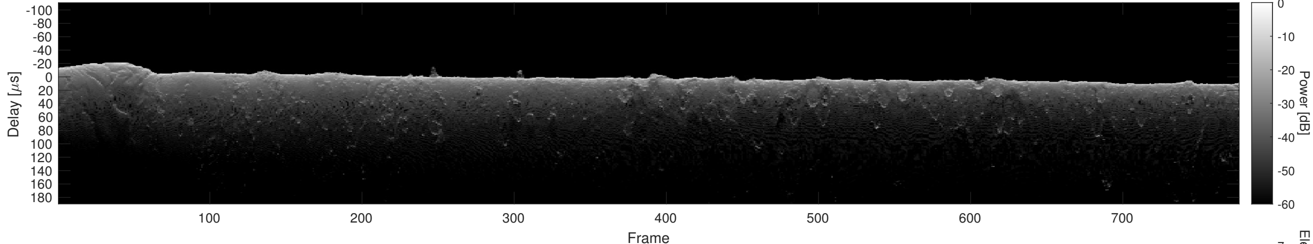
Orbit 14719, Cluttergram
