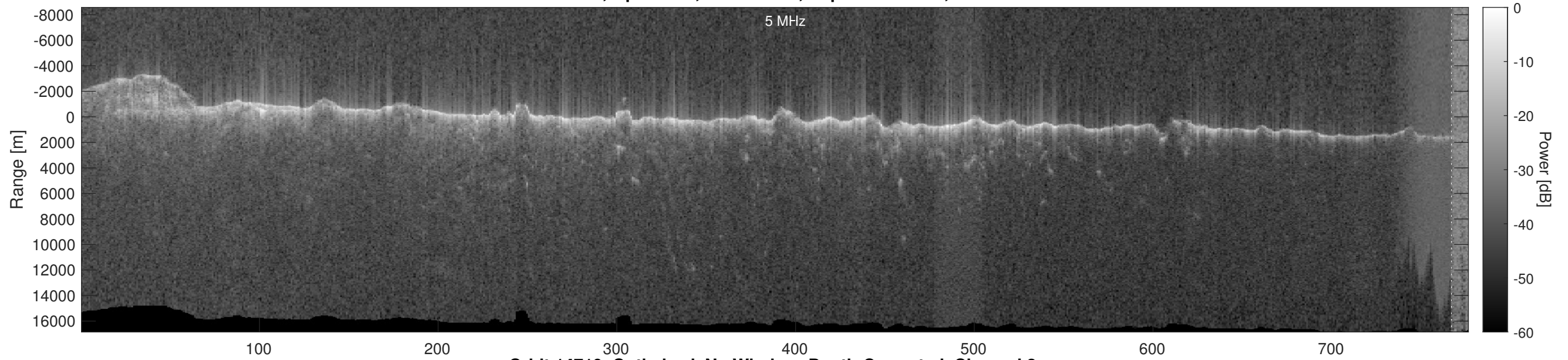
Orbit 14719, Optimized, No Window, Depth-Corrected, Channel 2
