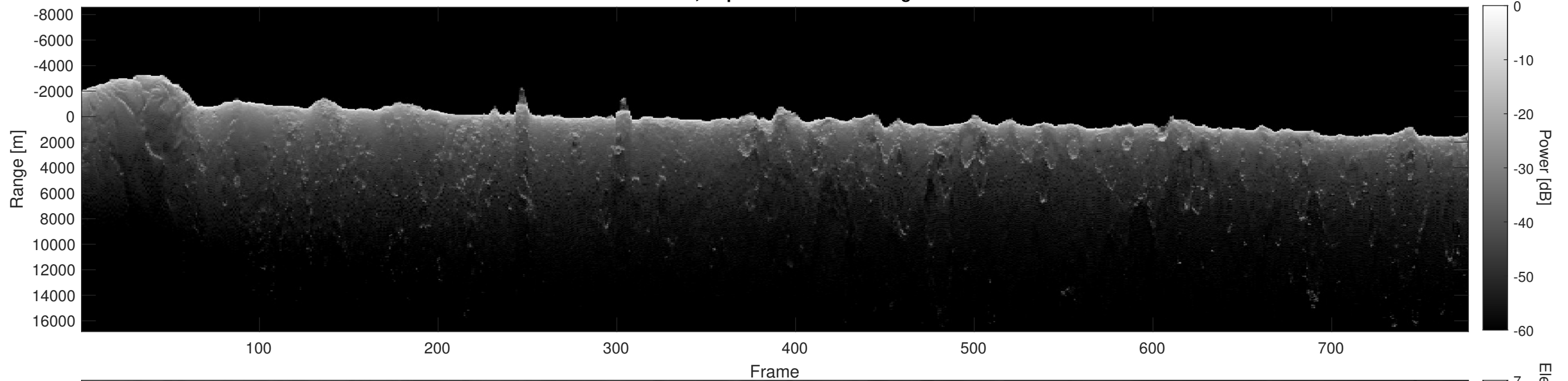
Orbit 14719, Depth-Corrected Cluttergram
