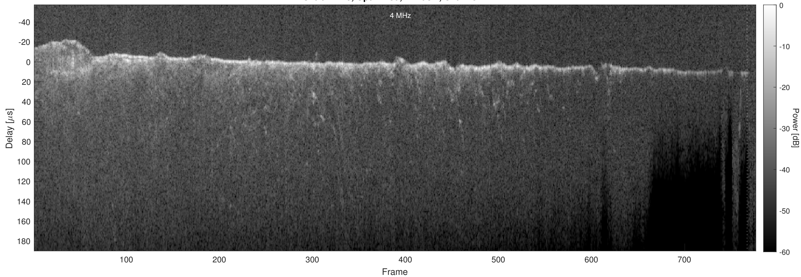
Orbit 14719, Optimized, Window, Channel 2
