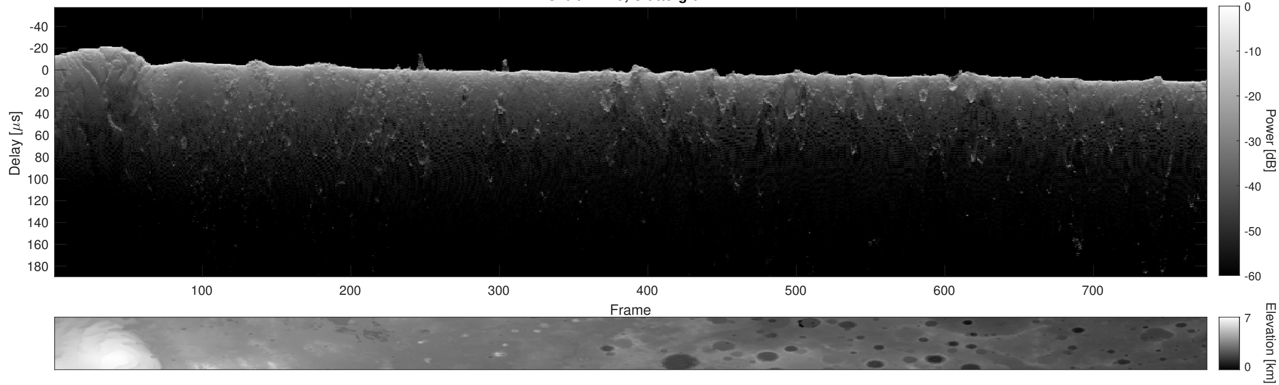
Orbit 14719, Cluttergram
