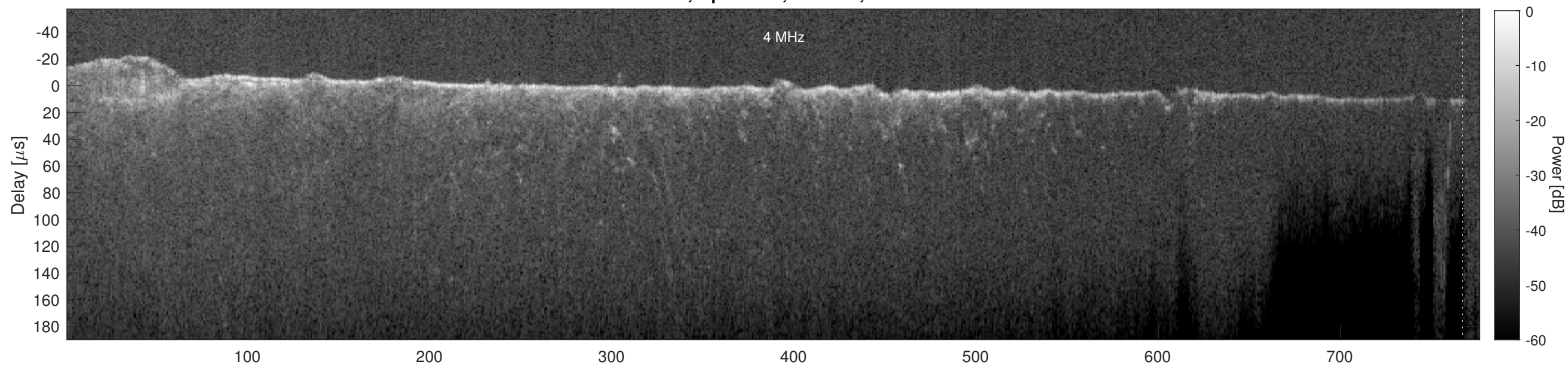
Orbit 14719, Cluttergram
