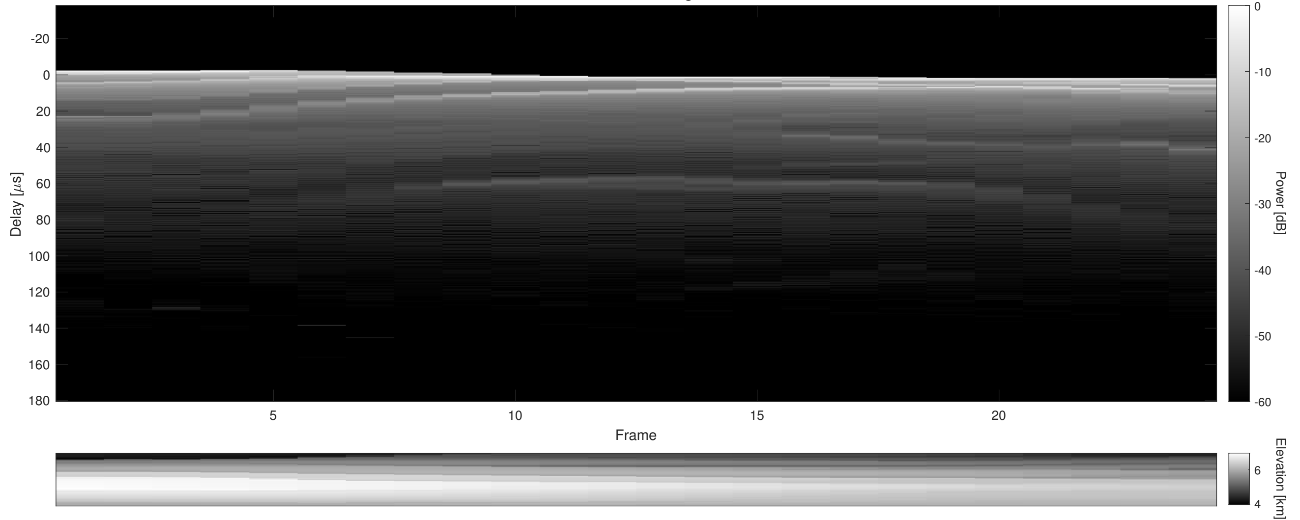
Orbit 14725, Cluttergram
