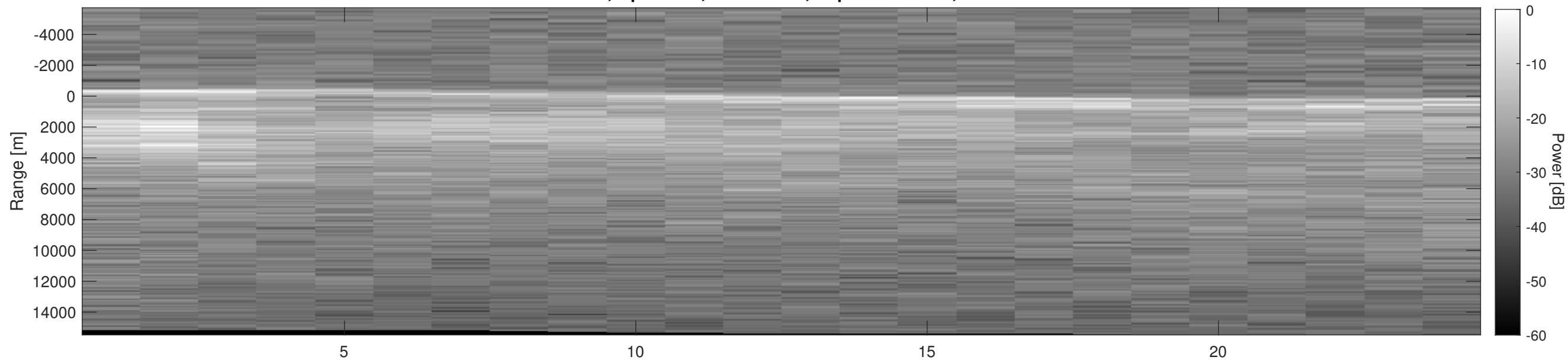
Orbit 14725, Depth-Corrected Cluttergram
