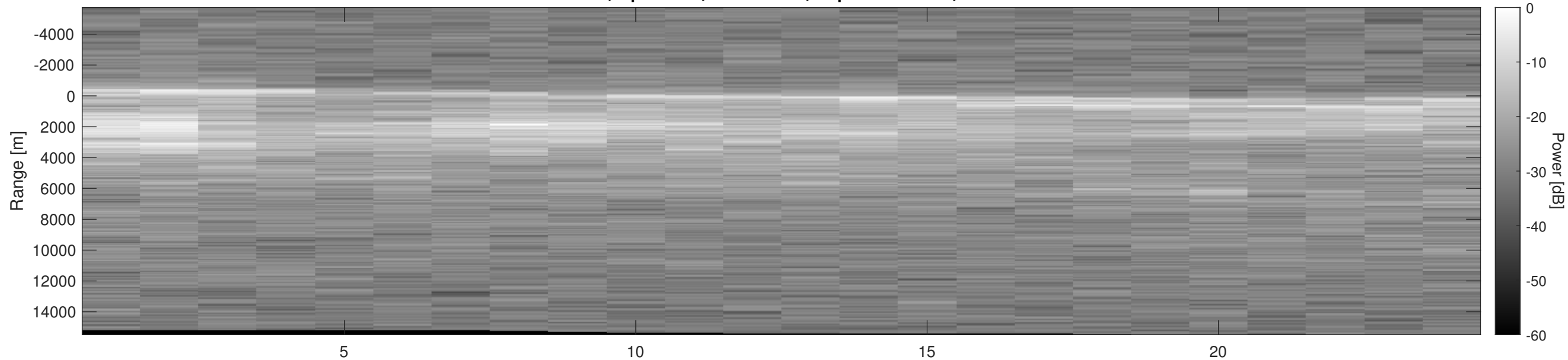
Orbit 14725, Optimized, No Window, Depth-Corrected, Channel 2
