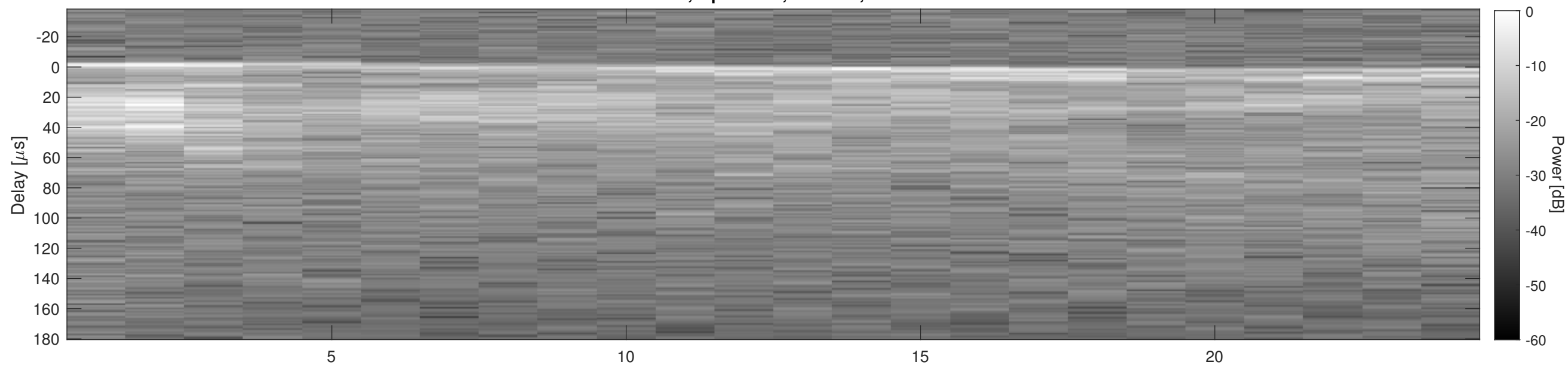
Orbit 14725, Cluttergram
