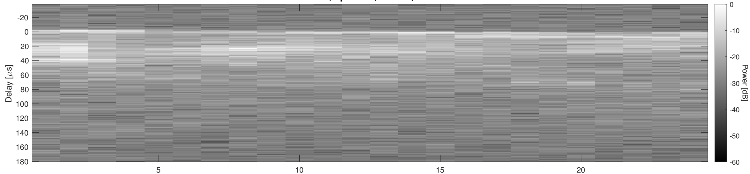
Orbit 14725, Optimized, Window, Channel 2
