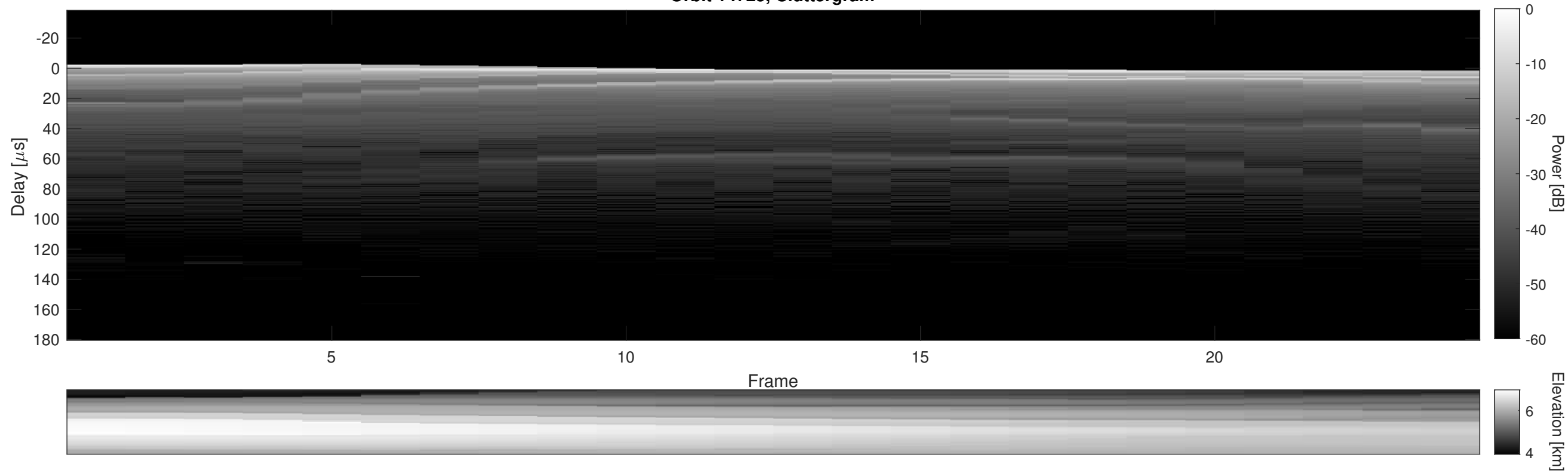
Orbit 14725, Cluttergram
