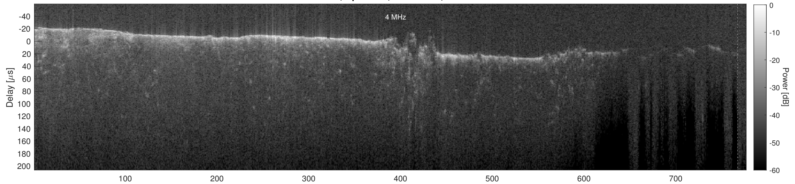
Orbit 14730, Cluttergram
