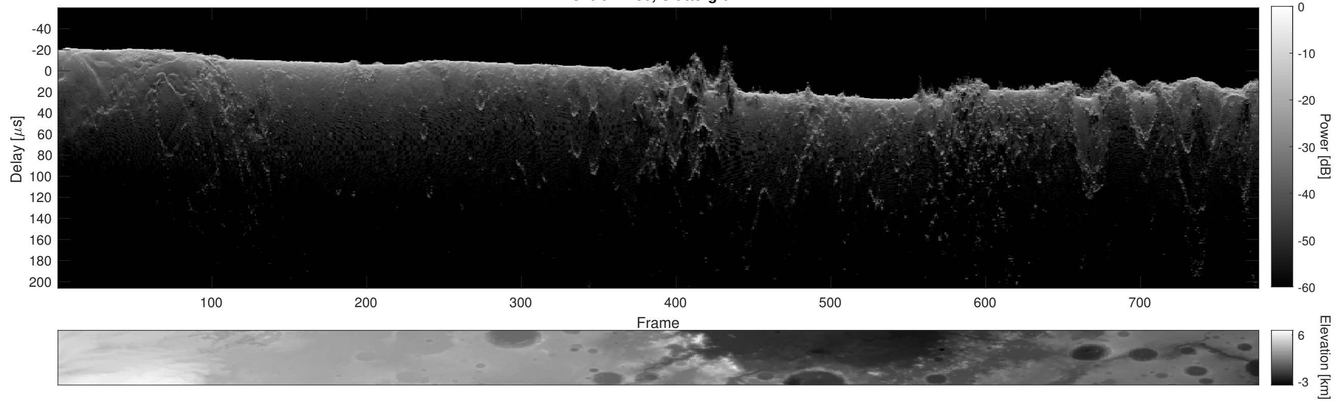
Orbit 14730, Cluttergram
