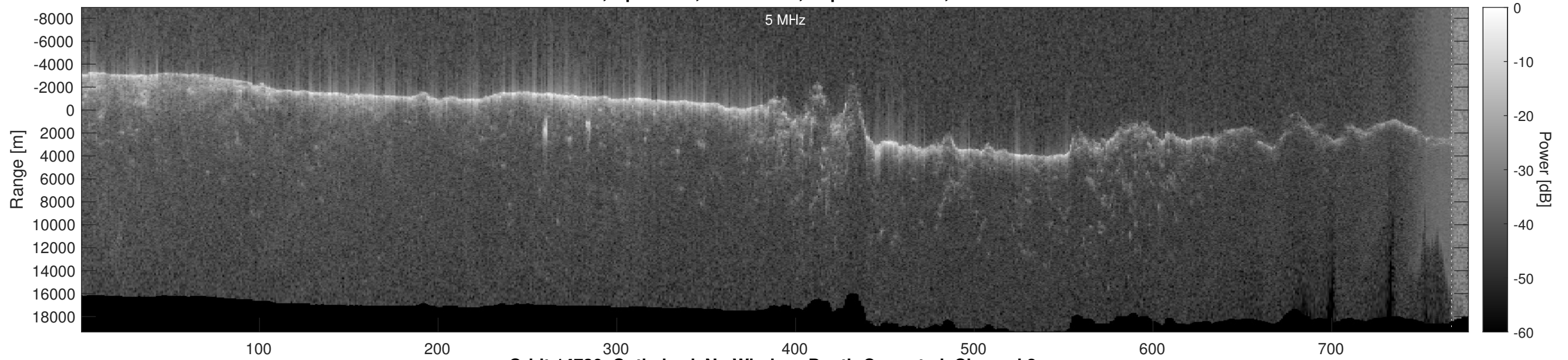
Orbit 14730, Optimized, No Window, Depth-Corrected, Channel 2
