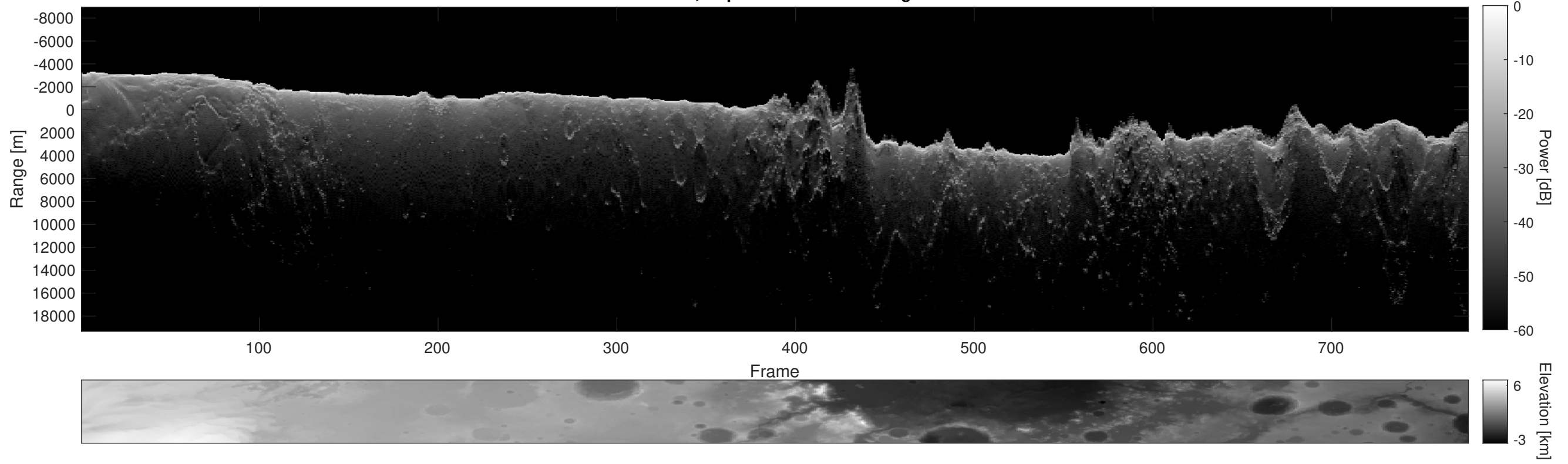
Orbit 14730, Depth-Corrected Cluttergram
