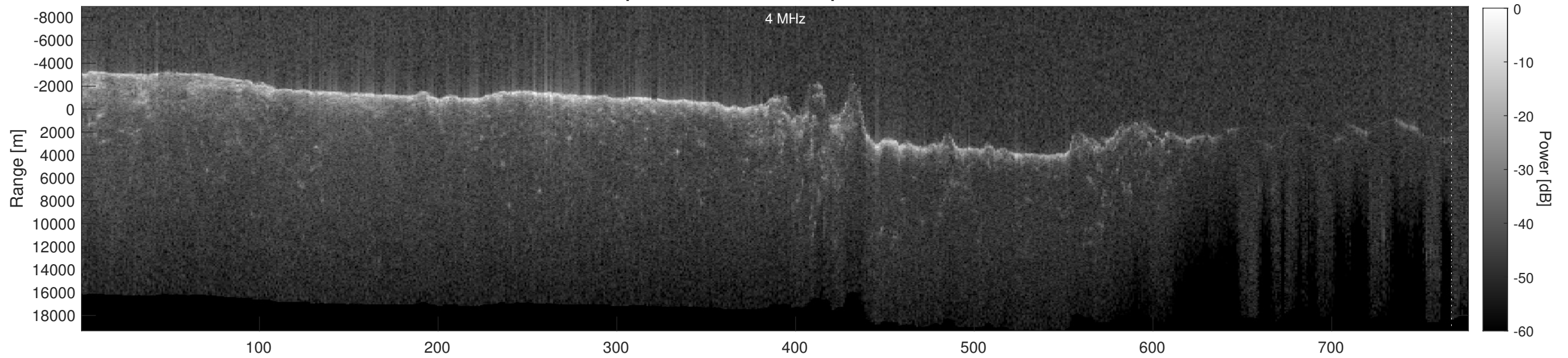
Orbit 14730, Depth-Corrected Cluttergram
