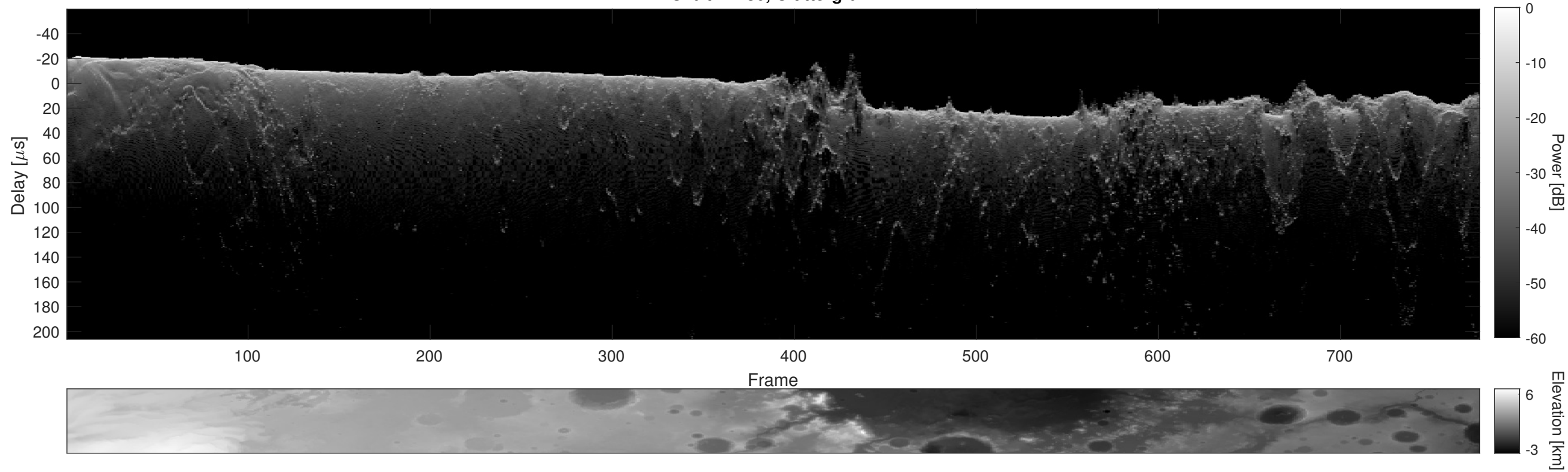
Orbit 14730, Cluttergram
