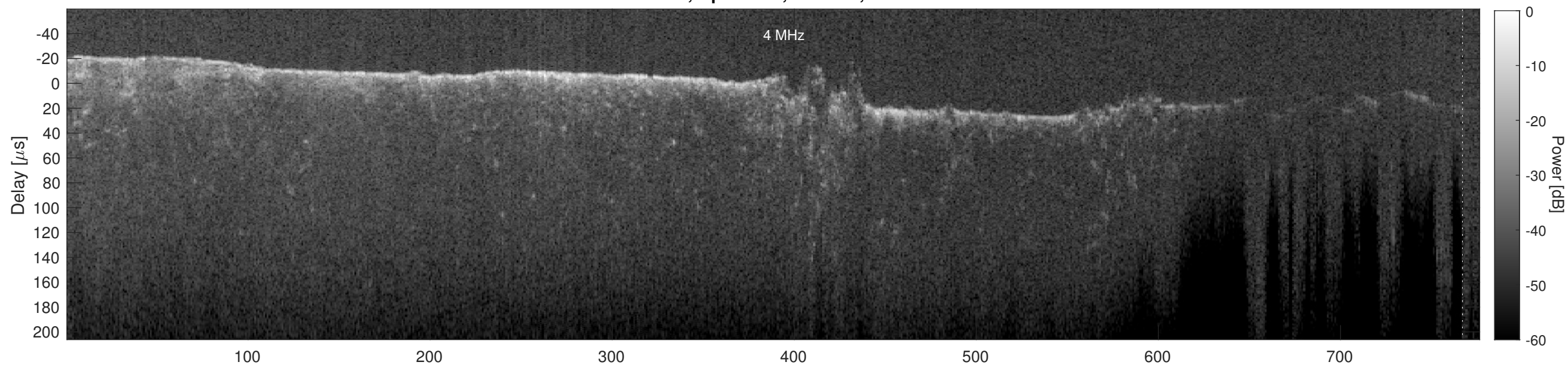
Orbit 14730, Cluttergram
