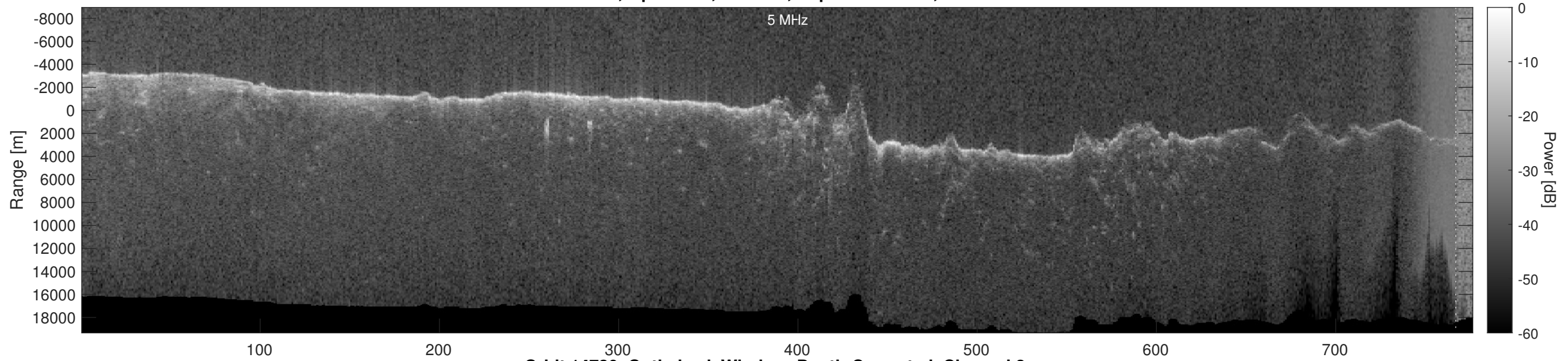
Orbit 14730, Optimized, Window, Depth-Corrected, Channel 2
