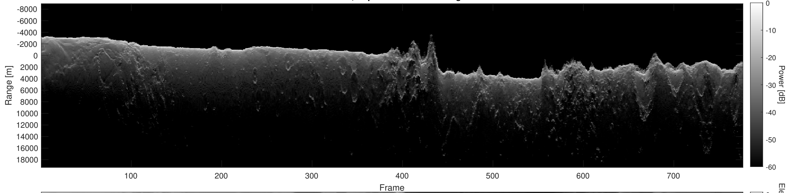
Orbit 14730, Depth-Corrected Cluttergram
