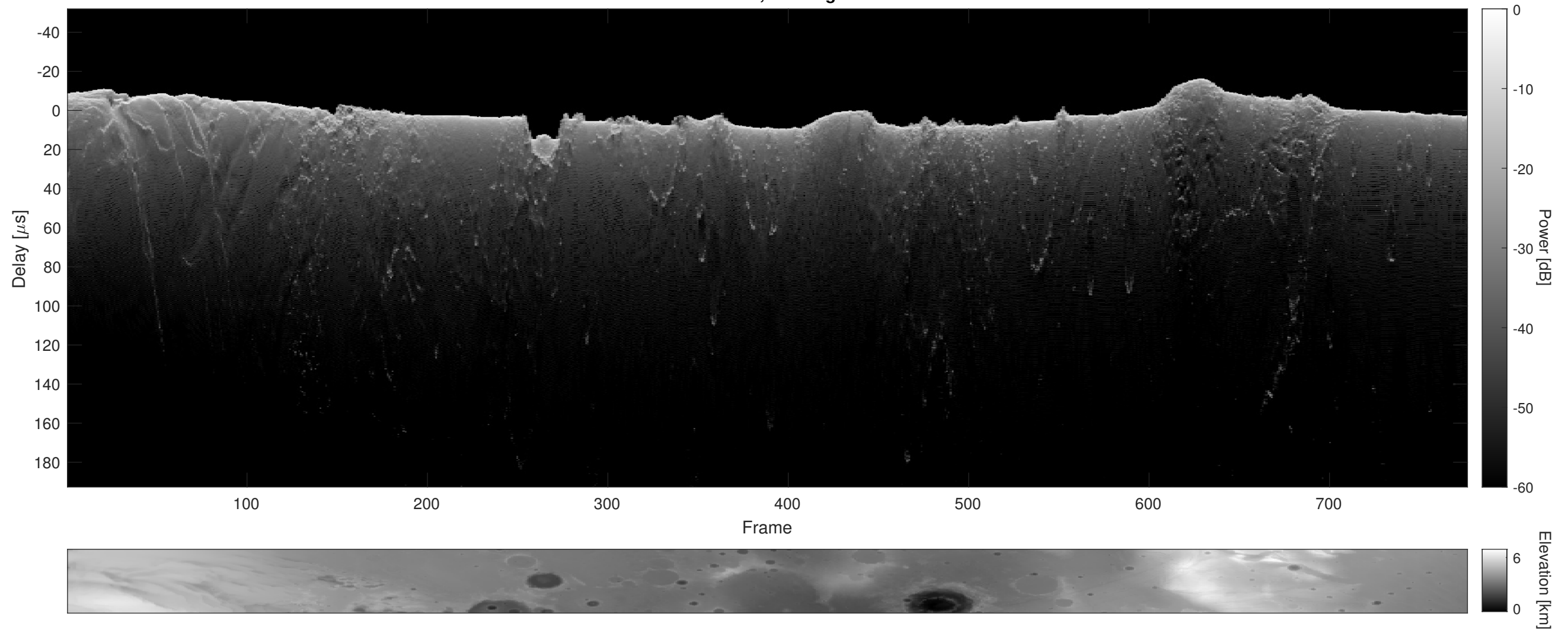
Orbit 14734, Cluttergram
