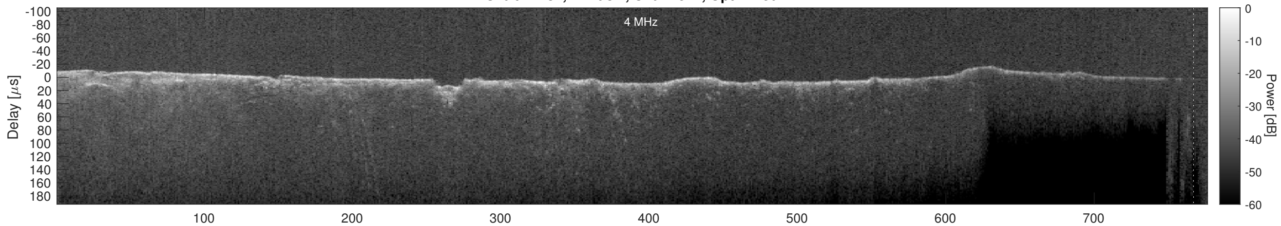
Orbit 14734, Cluttergram
