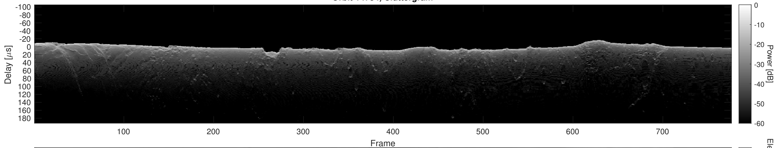
Orbit 14734, Cluttergram
