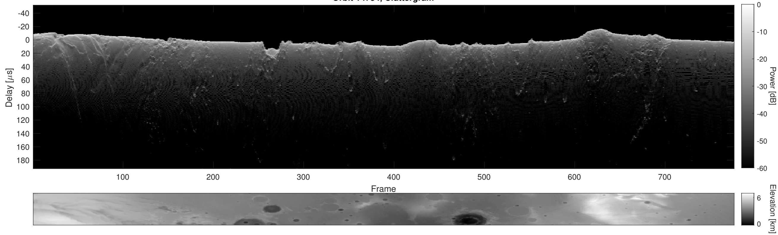
Orbit 14734, Cluttergram
