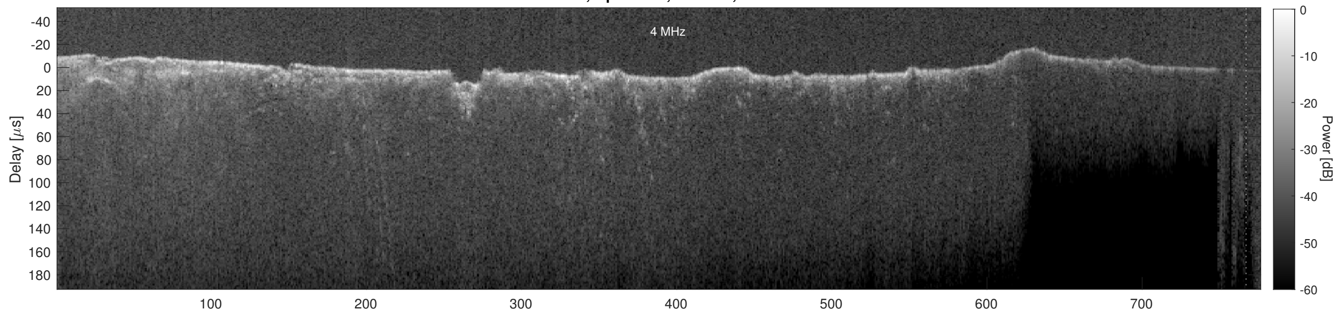
Orbit 14734, Cluttergram
