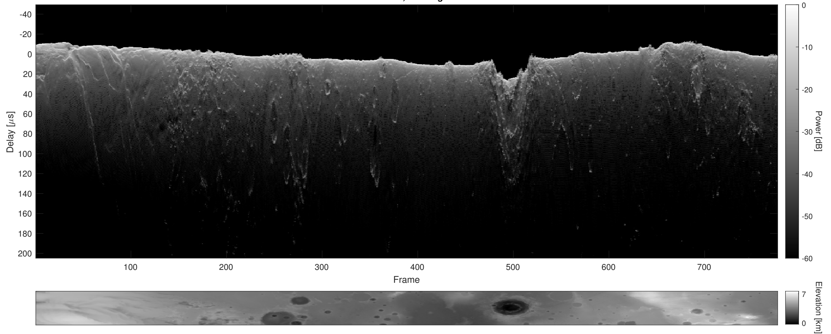
Orbit 14741, Cluttergram
