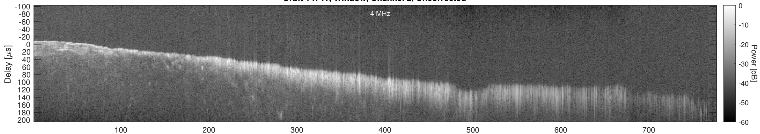
Orbit 14741, Window, Channel 2, Chapman
