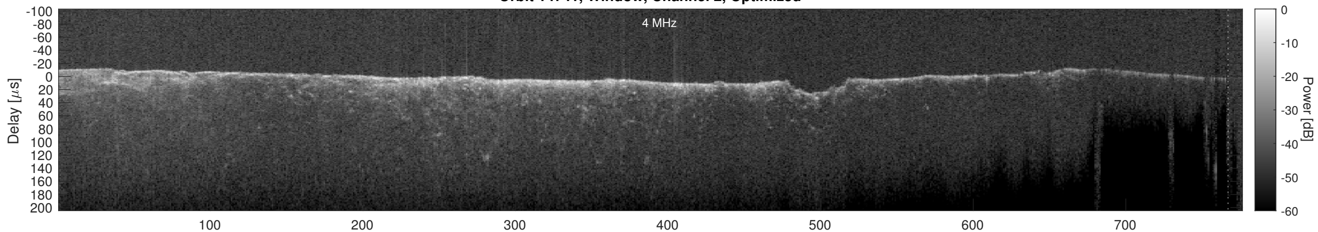
Orbit 14741, Cluttergram
