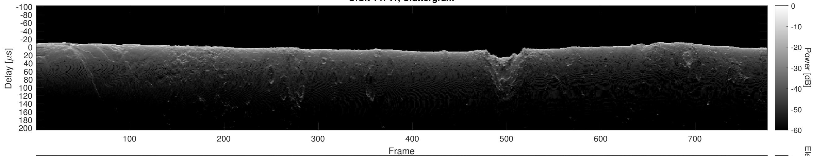
Orbit 14741, Cluttergram
