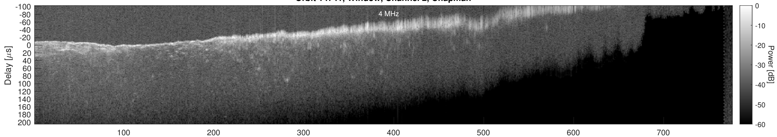
Orbit 14741, Window, Channel 2, Optimized
