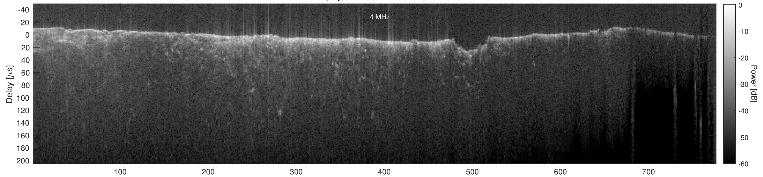
Orbit 14741, Cluttergram
