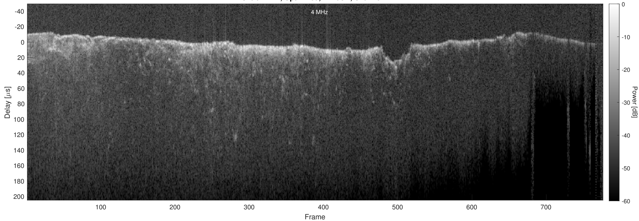
Orbit 14741, Optimized, Window, Channel 2
