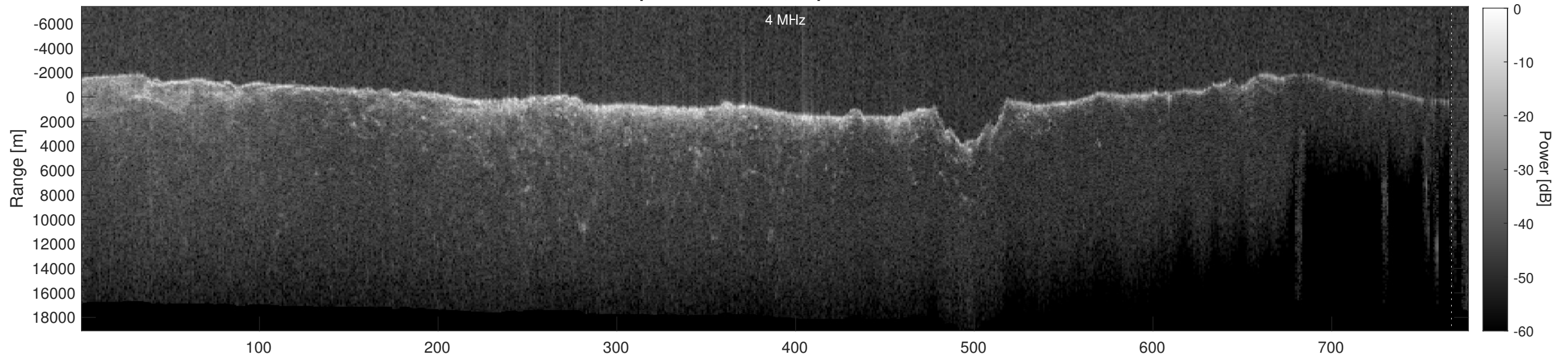
Orbit 14741, Depth-Corrected Cluttergram
