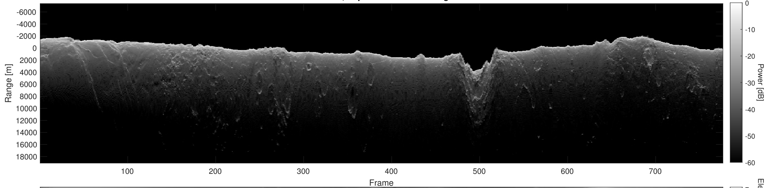
Orbit 14741, Depth-Corrected Cluttergram
