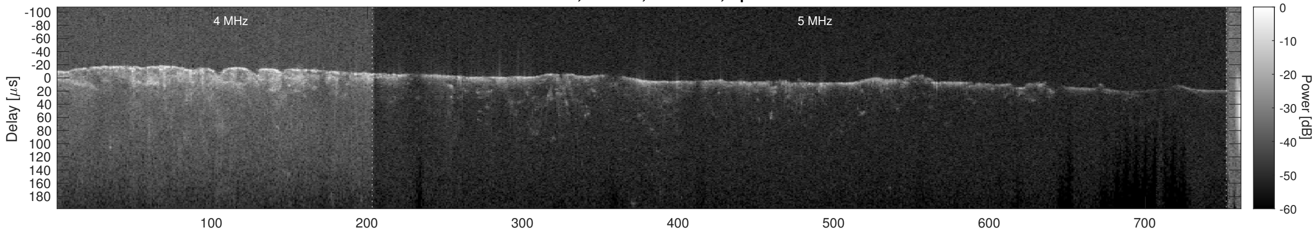
Orbit 14749, Cluttergram
