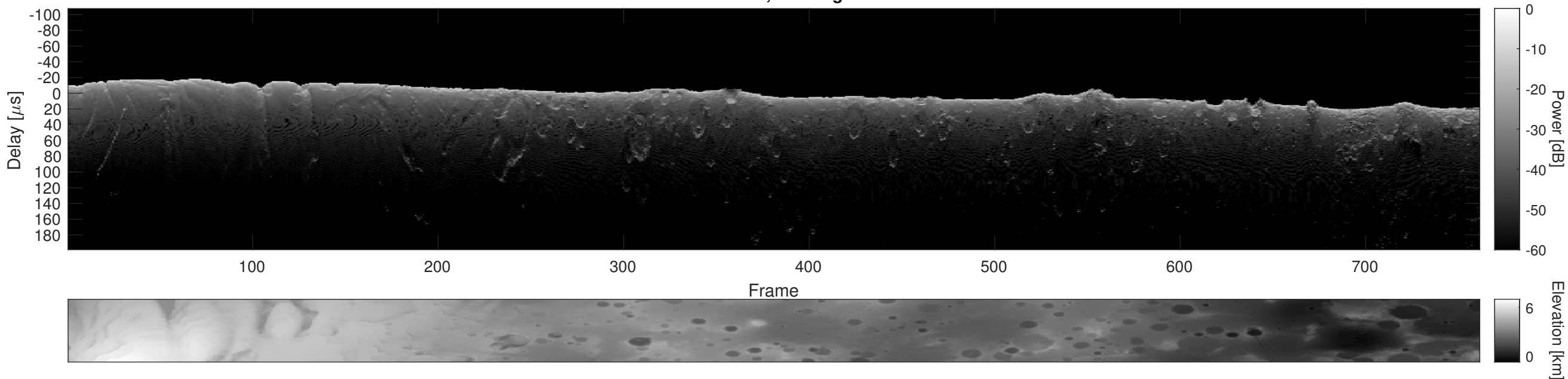
Orbit 14749, Cluttergram
