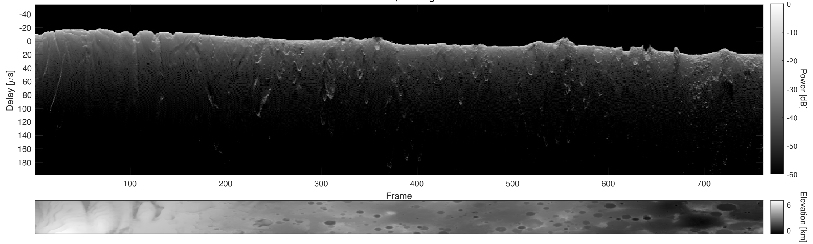
Orbit 14749, Cluttergram
