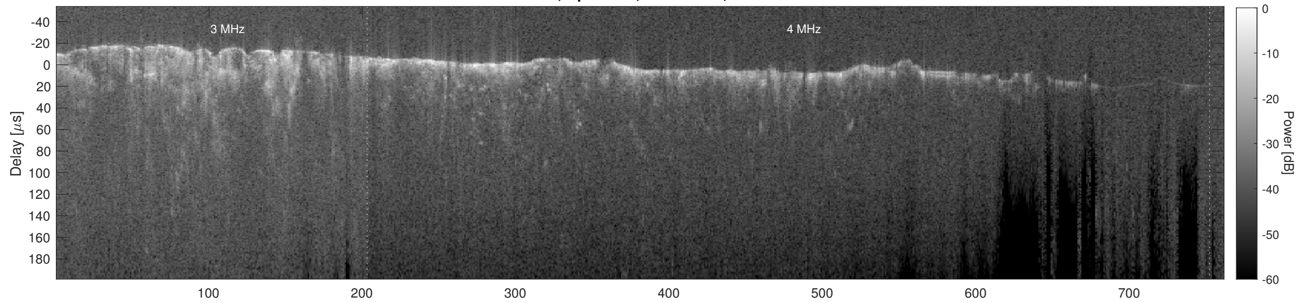
Orbit 14749, Cluttergram
