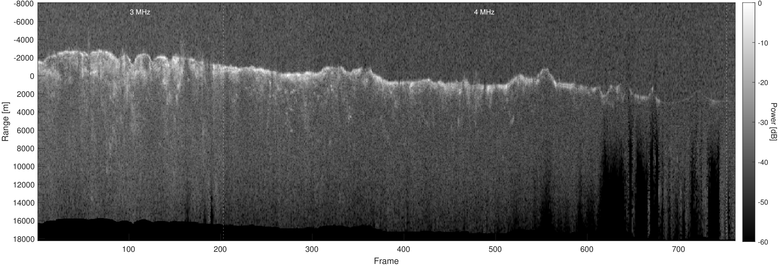
Orbit 14749, Optimized, Window, Depth-Corrected, Channel 2
