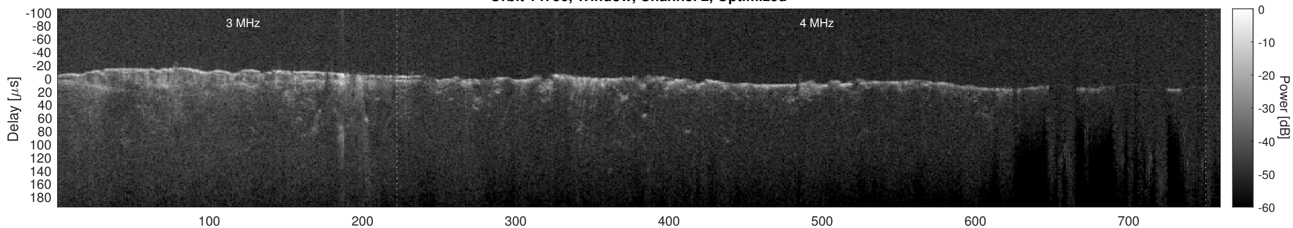
Orbit 14756, Cluttergram
