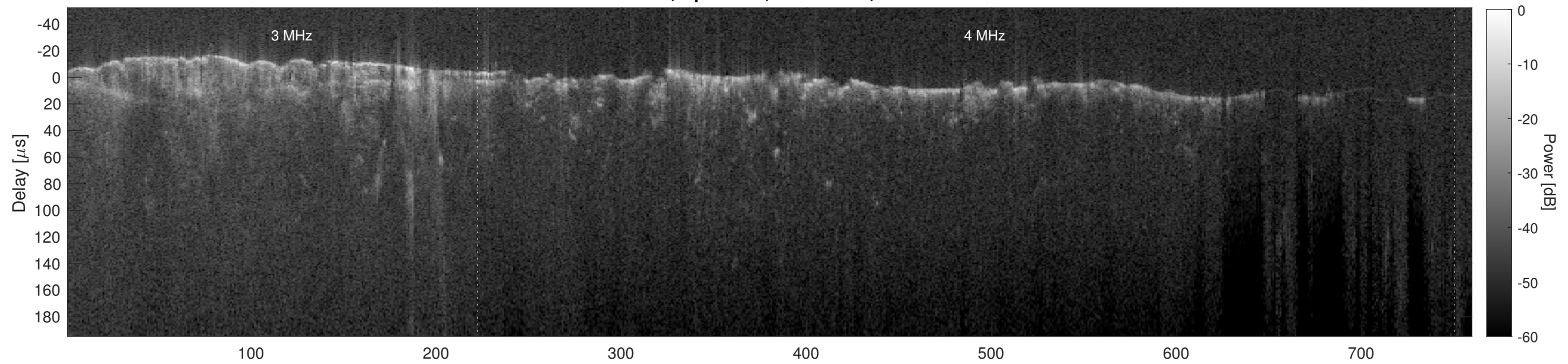
Orbit 14756, Cluttergram
