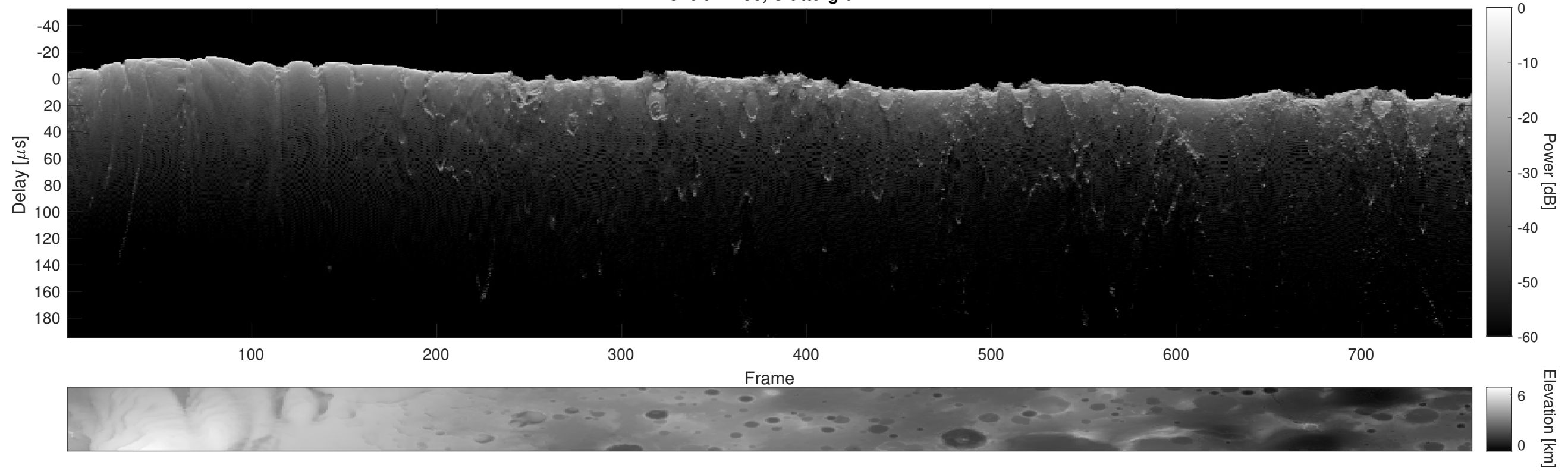
Orbit 14756, Cluttergram
